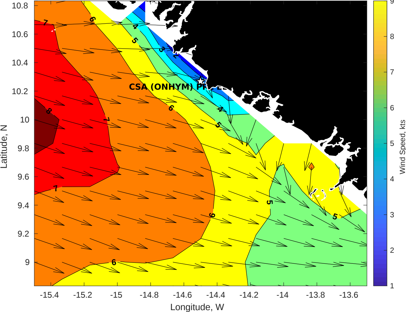
GFS Winds (kts) for CSA (ONHYM) PPL EBS - Guinea at 12-Dec-2025 09:00:00
