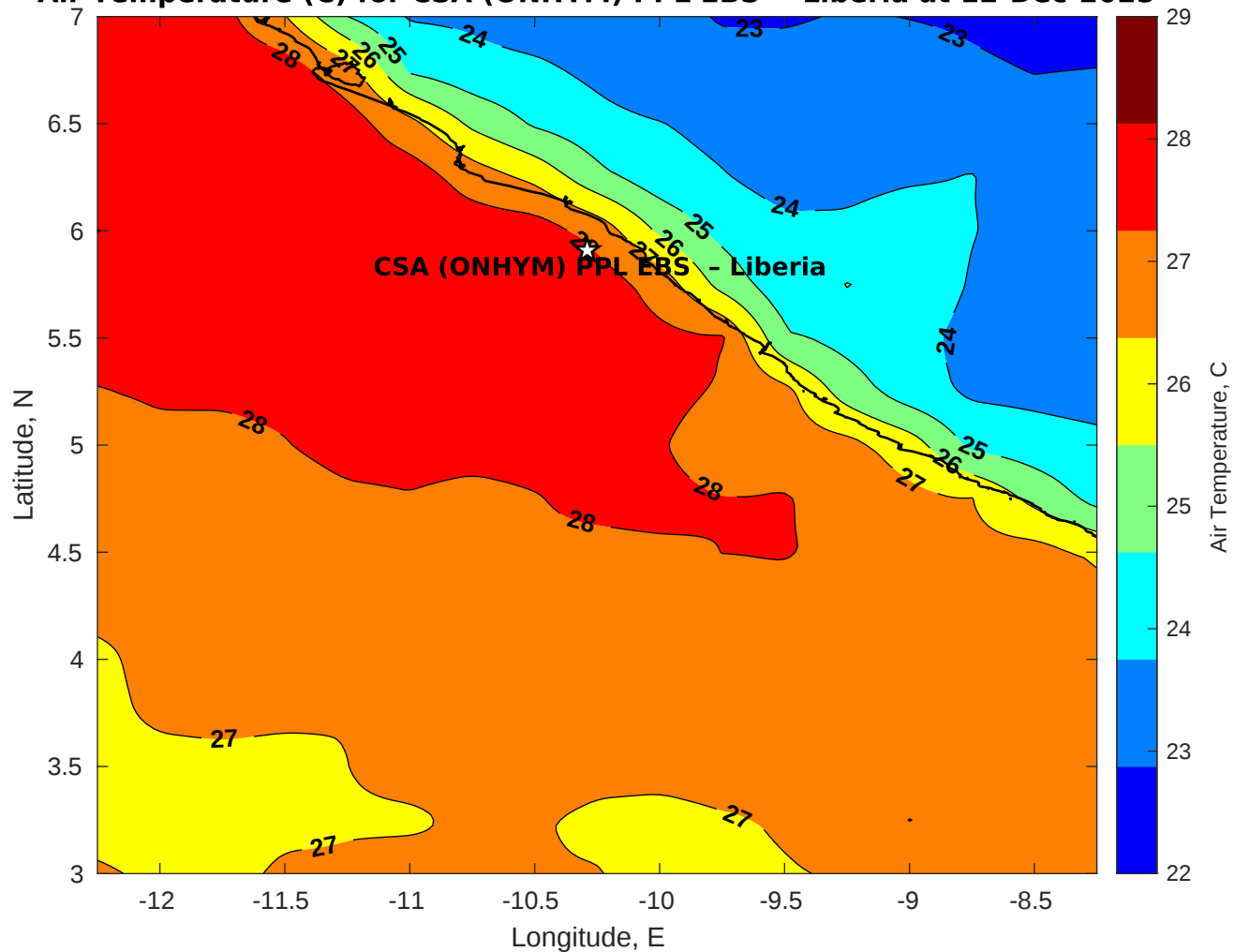
Air Temperature (C) for CSA (ONHYM) PPL EBS - Liberia at 12-Dec-2025
