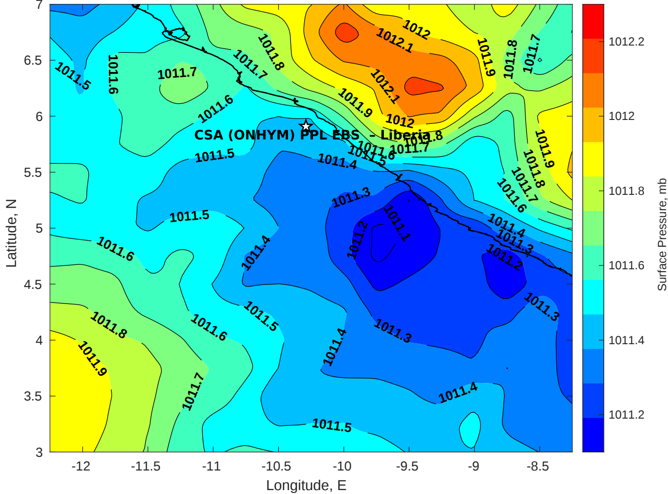
Surface Pressure (mb) for CSA (ONHYM) PPL EBS - Liberia at 14-Dec-2025 00:00:00
