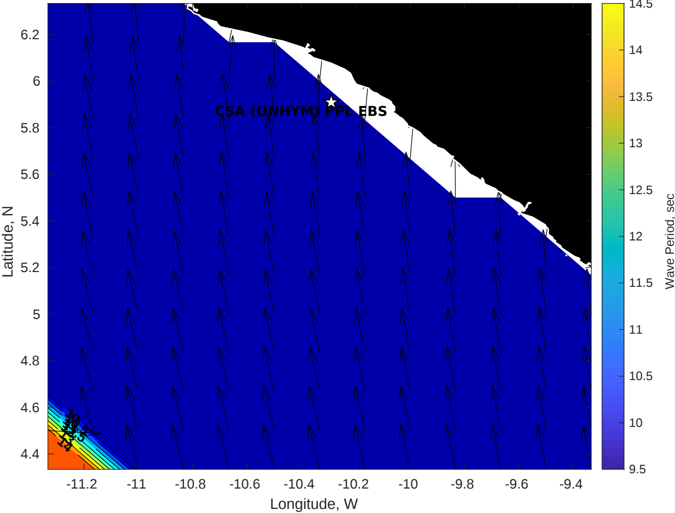
GFS Wave Period (sec) for CSA (ONHYM) PPL EBS - Liberia at 12-Dec-2025 09:00:00
