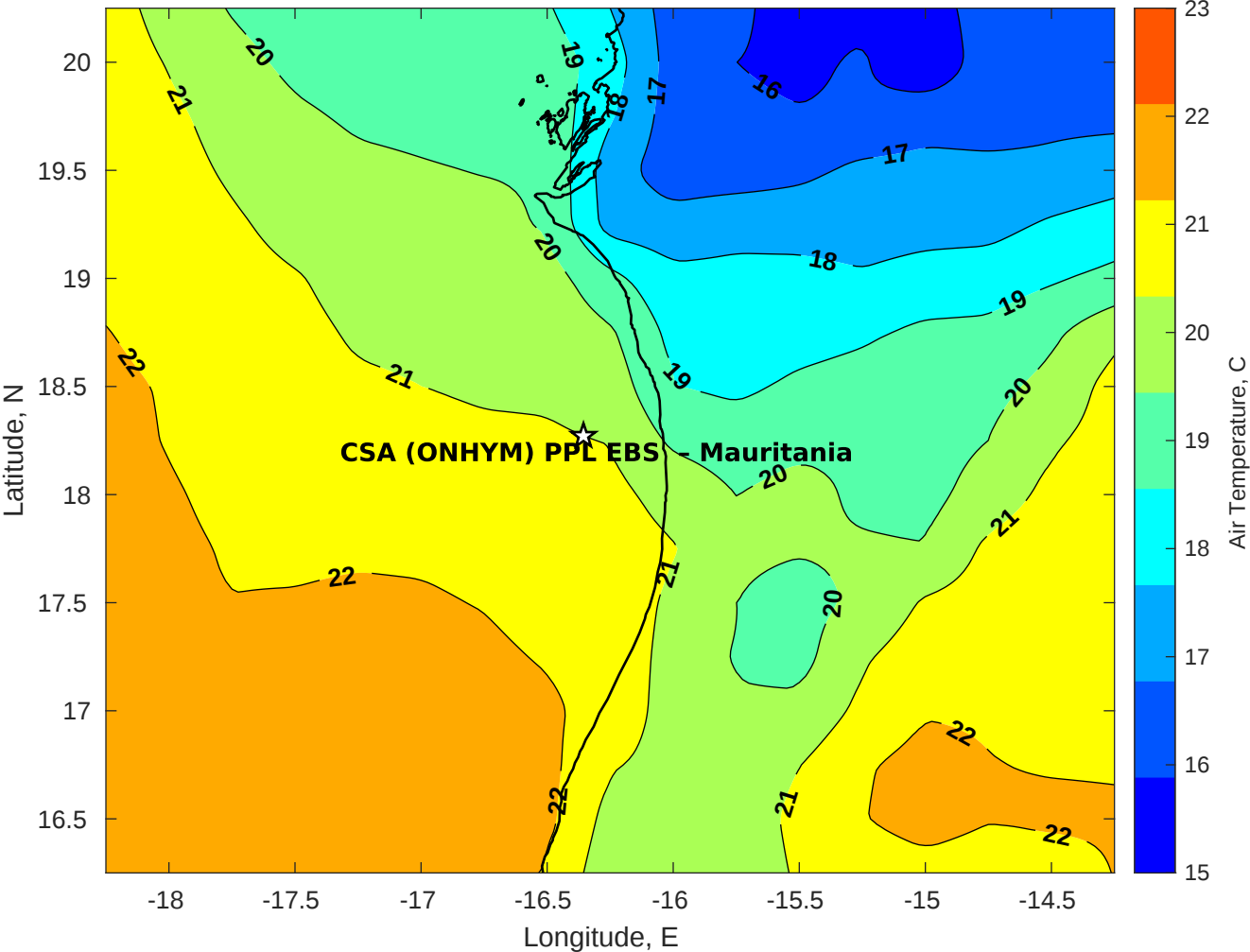
Air Temperature (C) for CSA (ONHYM) PPL EBS - Mauritania at 12-Dec-2025
