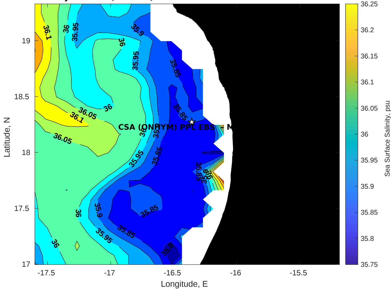
Surface Salinity for CSA (ONHYM) PPL EBS - Mauritania at 11-Dec-2025 00:00:00
