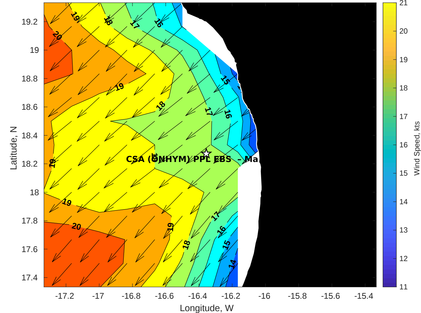
GFS Winds (kts) for CSA (ONHYM) PPL EBS - Mauritania at 12-Dec-2025 09:00:00
