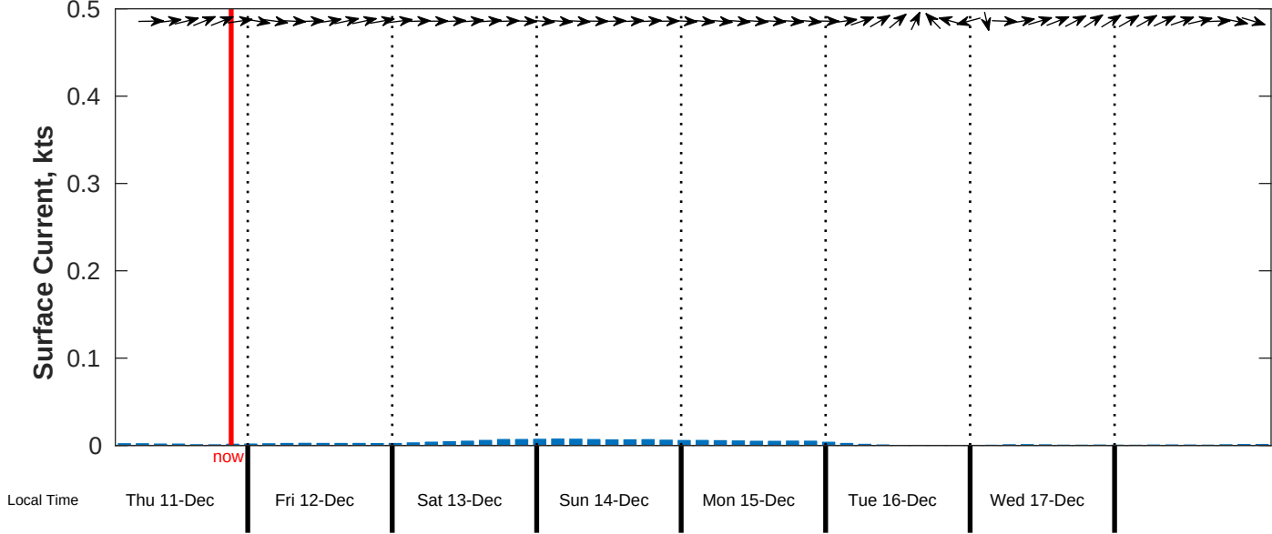
Surface Current Forecast for CSA (ONHYM) PPL EBS - Mauritania from 11-Dec-2025 00:00:00 to 19-Dec-2025 00:00:00
