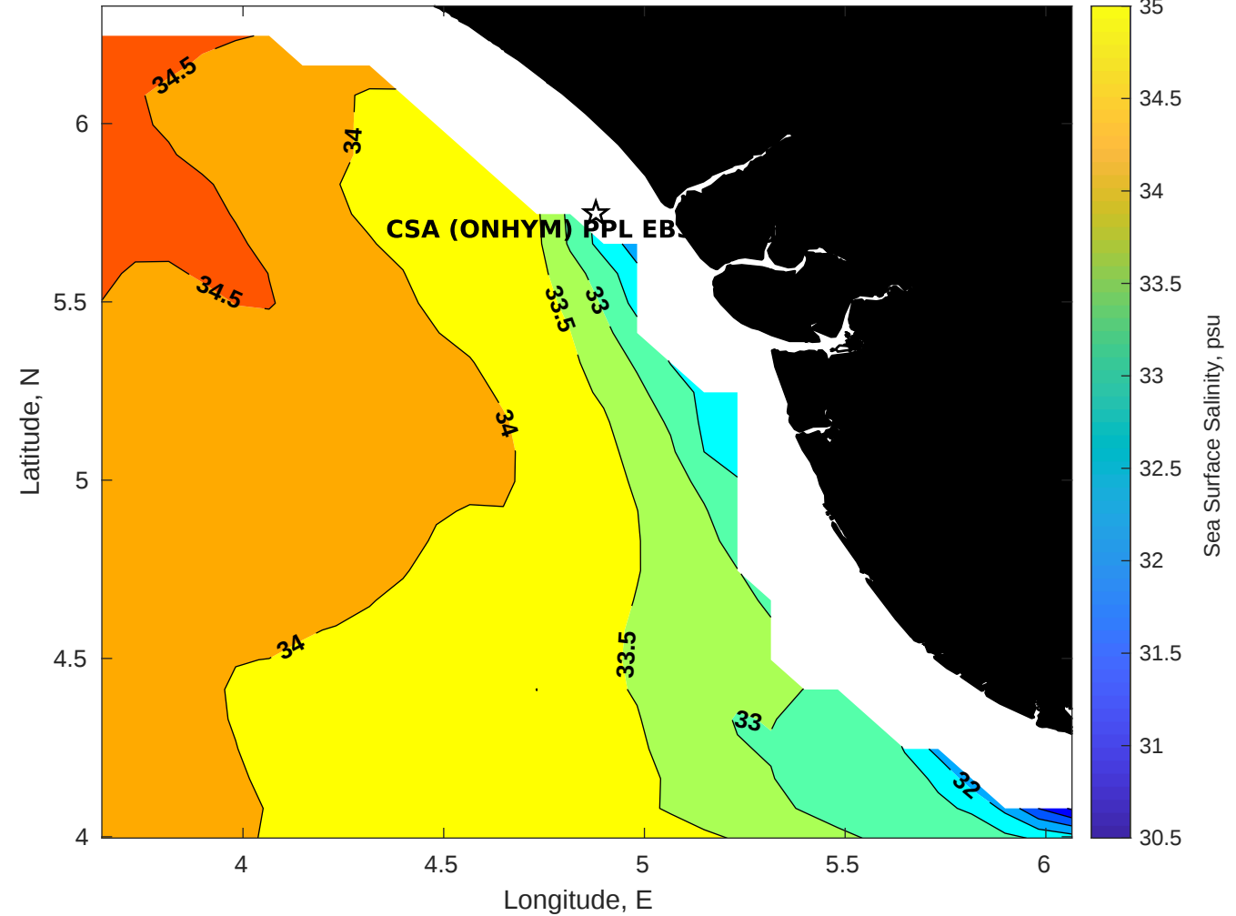
Surface Salinity for CSA (ONHYM) PPL EBS - Nigeria at 11-Dec-2025 00:00:00
