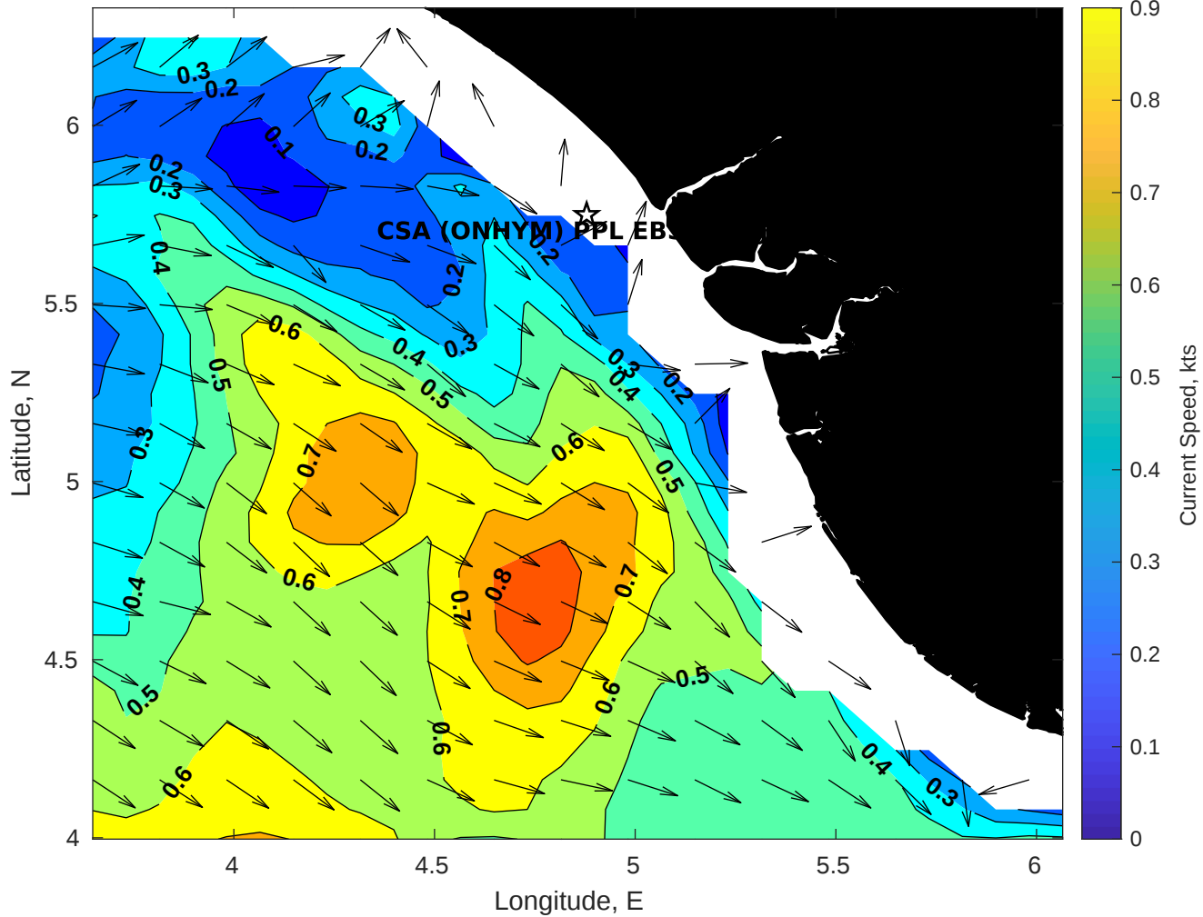
Surface Currents for CSA (ONHYM) PPL EBS - Nigeria at 11-Dec-2025 00:00:00
