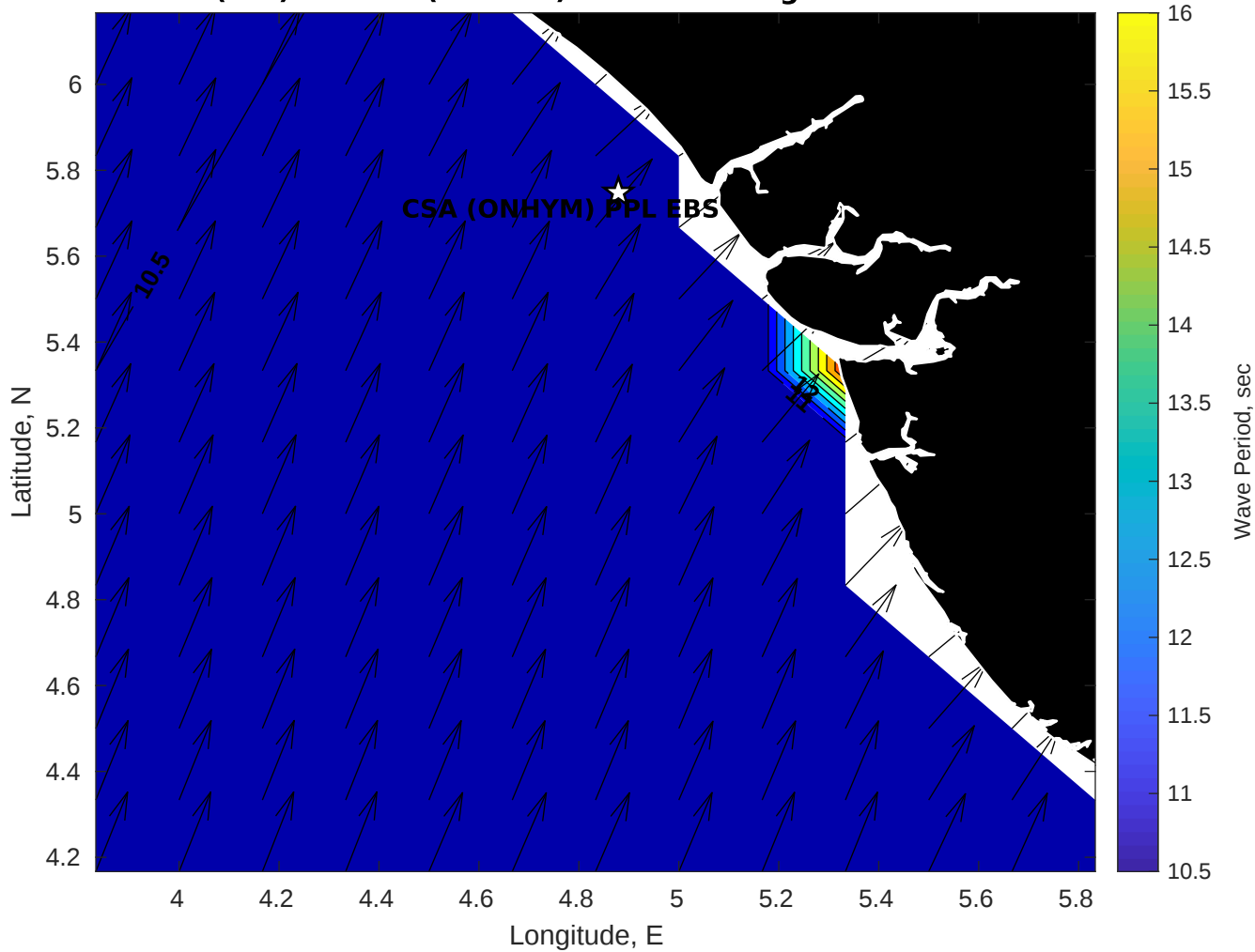
GFS Wave Period (sec) for CSA (ONHYM) PPL EBS - Nigeria at 12-Dec-2025 09:00:00
