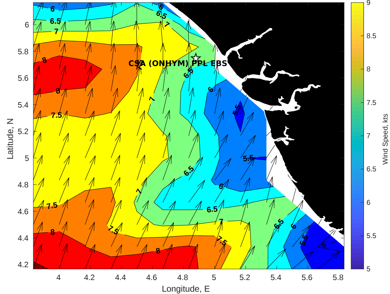
GFS Winds (kts) for CSA (ONHYM) PPL EBS - Nigeria at 12-Dec-2025 09:00:00
