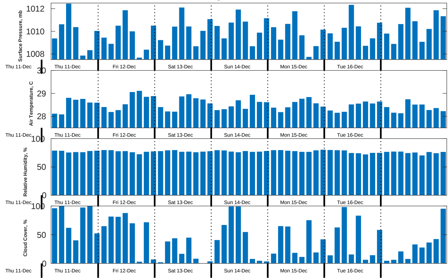
Met Forecast for CSA (ONHYM) PPL EBS - Nigeria from 12-Dec-2025 00:00:00 to 19-Dec-2025 00:00:00
