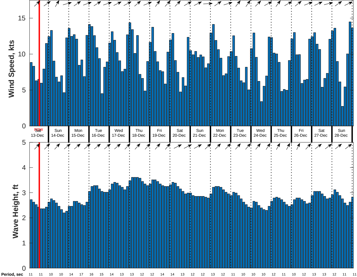
Wind & Wave Forecast for CSA (ONHYM) PPL EBS - Nigeria from 12-Dec-2025 02:00:00 to 28-Dec-2025 02:00:00
