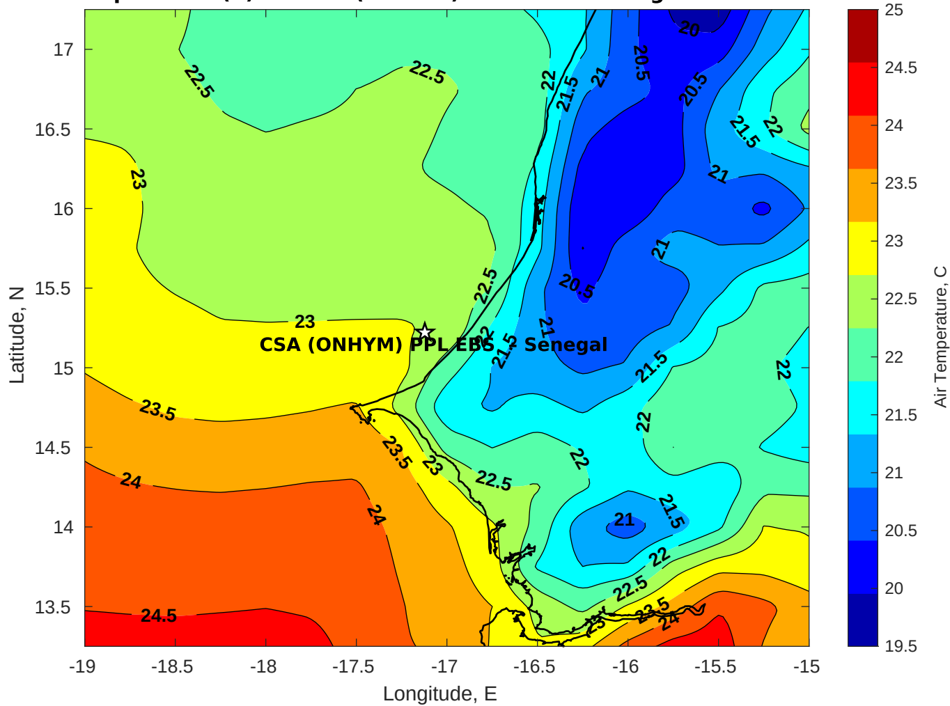
Air Temperature (C) for CSA (ONHYM) PPL EBS - Senegal at 12-Dec-2025
