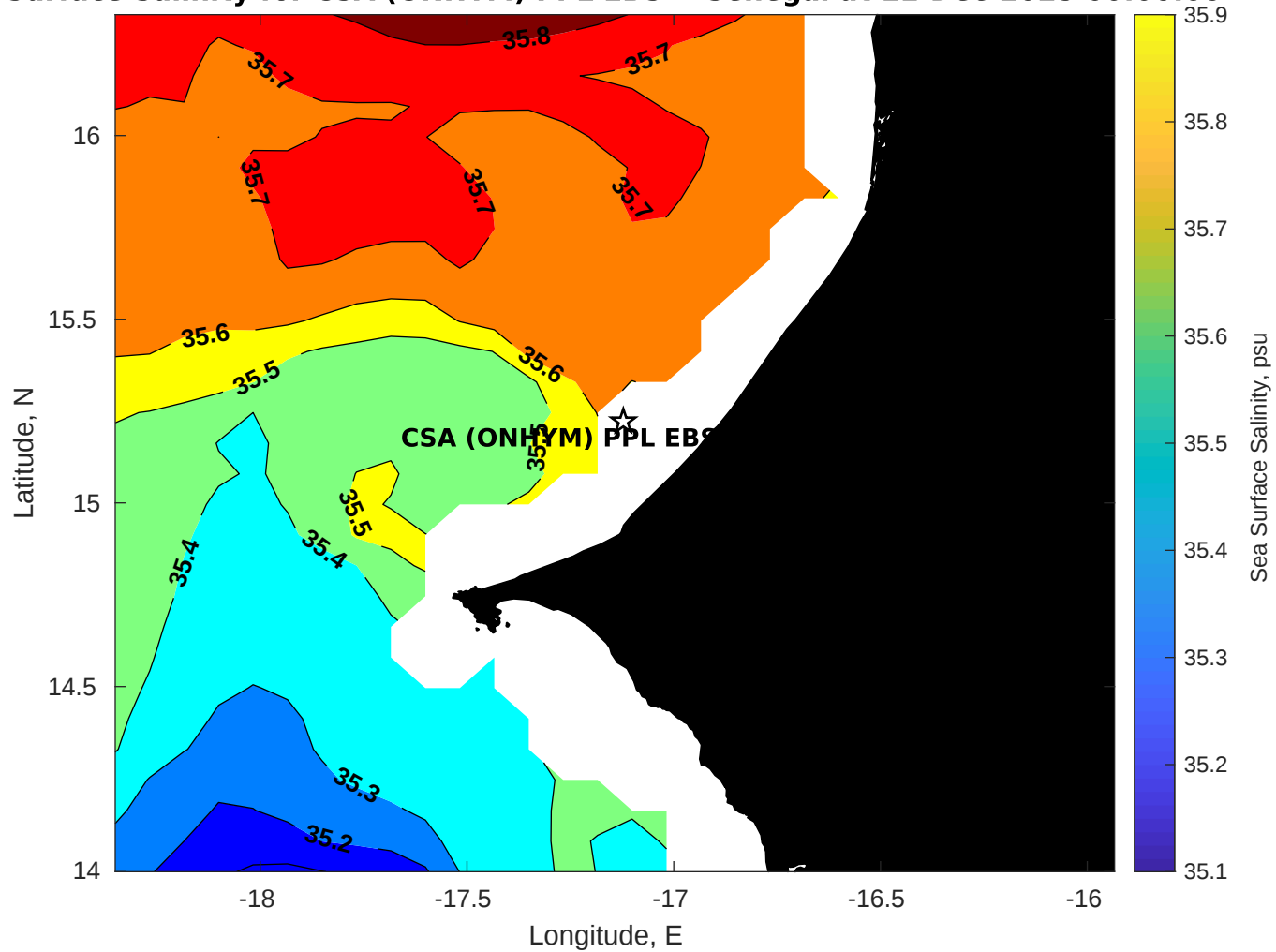
Surface Salinity for CSA (ONHYM) PPL EBS - Senegal at 11-Dec-2025 00:00:00
