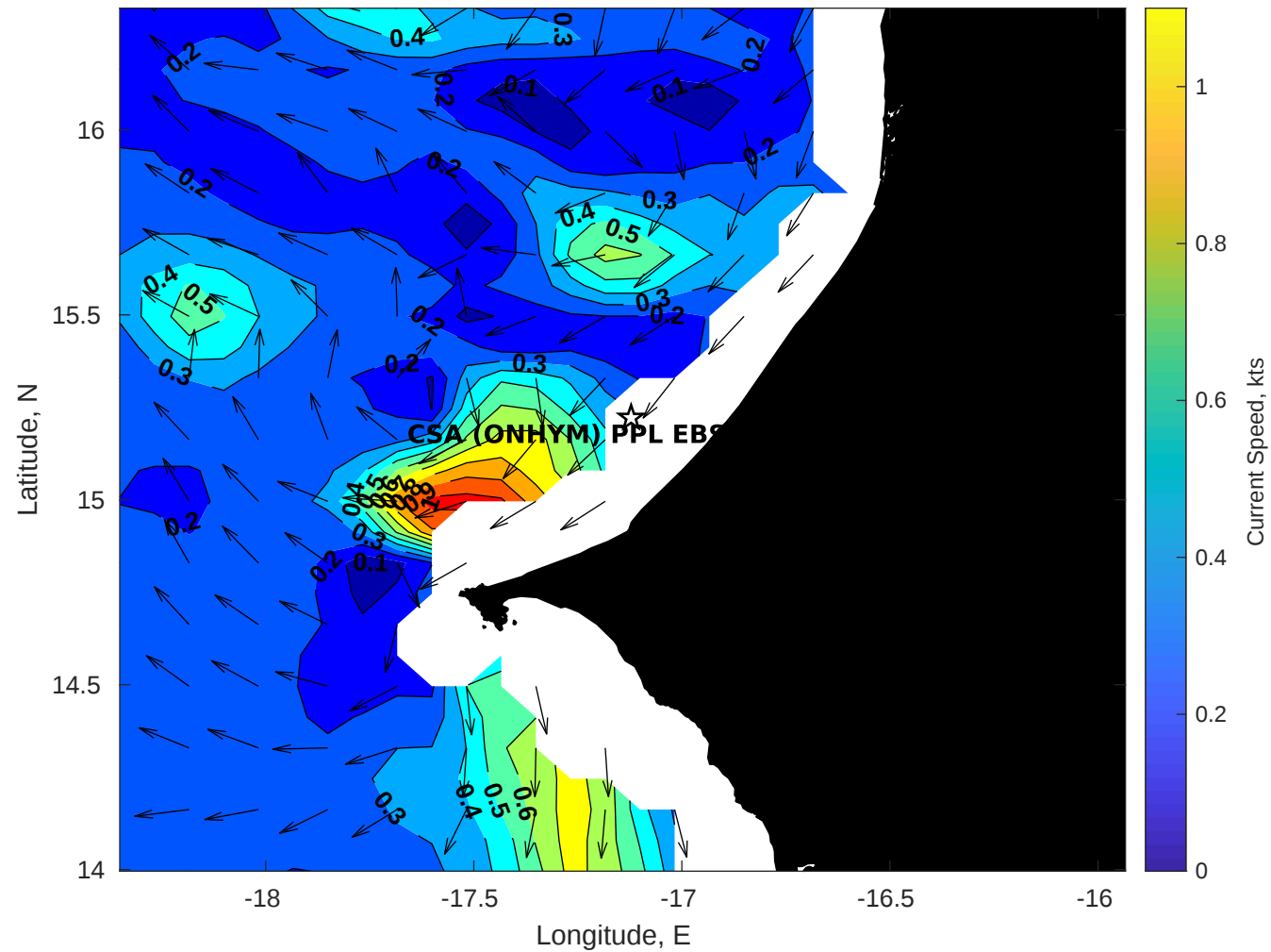
Surface Currents for CSA (ONHYM) PPL EBS - Senegal at 11-Dec-2025 00:00:00
