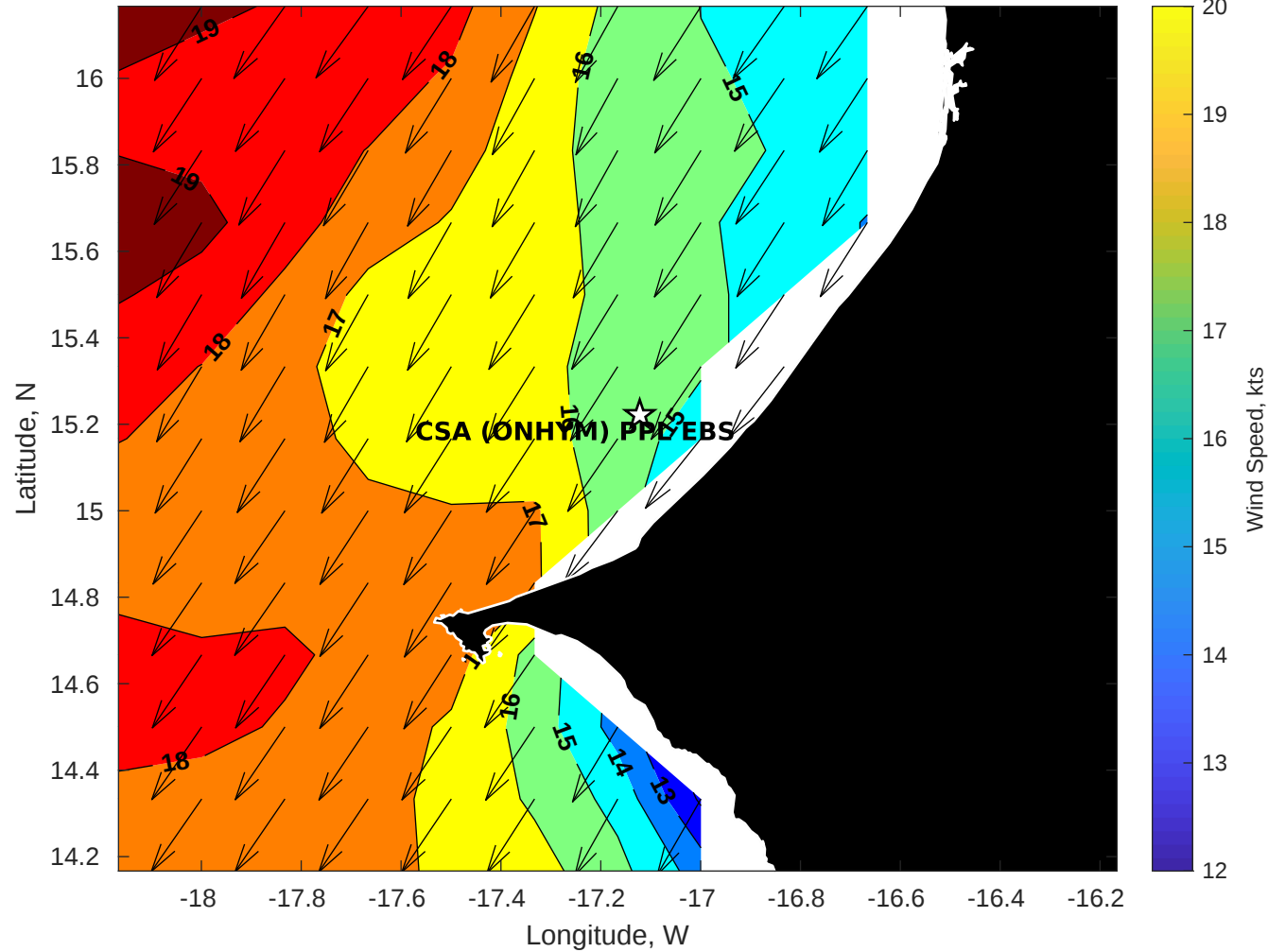
GFS Winds (kts) for CSA (ONHYM) PPL EBS - Senegal at 12-Dec-2025 09:00:00
