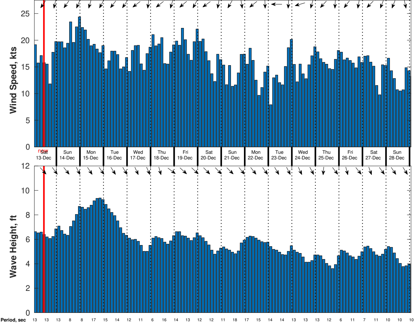
Wind & Wave Forecast for CSA (ONHYM) PPL EBS - Senegal from 12-Dec-2025 01:00:00 to 28-Dec-2025 01:00:00
