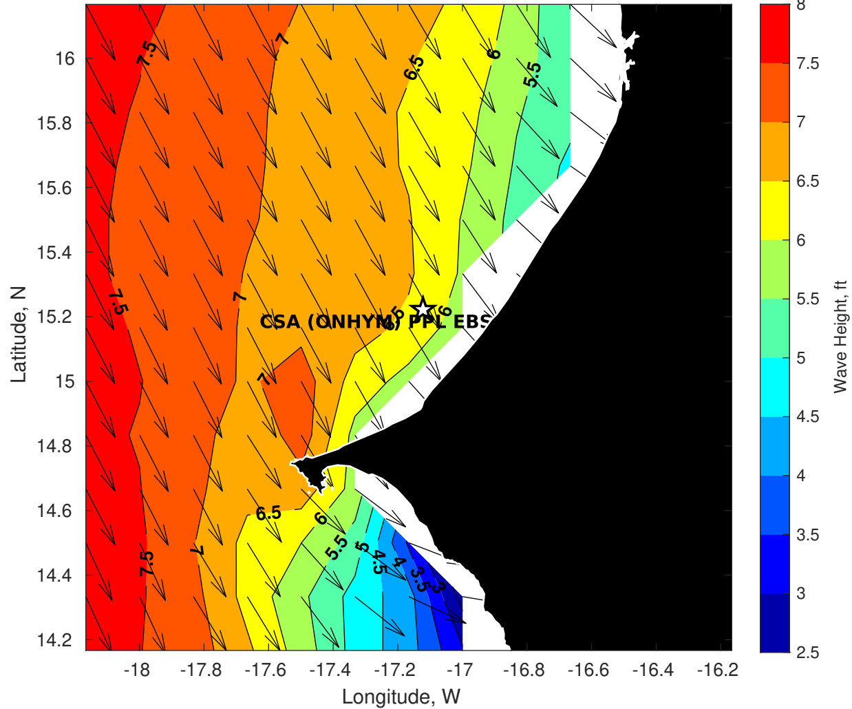
GFS Wave Height (ft) for CSA (ONHYM) PPL EBS - Senegal at 12-Dec-2025 09:00:00
