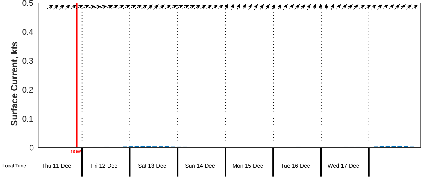
Surface Current Forecast for CSA (ONHYM) PPL EBS - Senegal from 11-Dec-2025 00:00:00 to 19-Dec-2025 00:00:00
