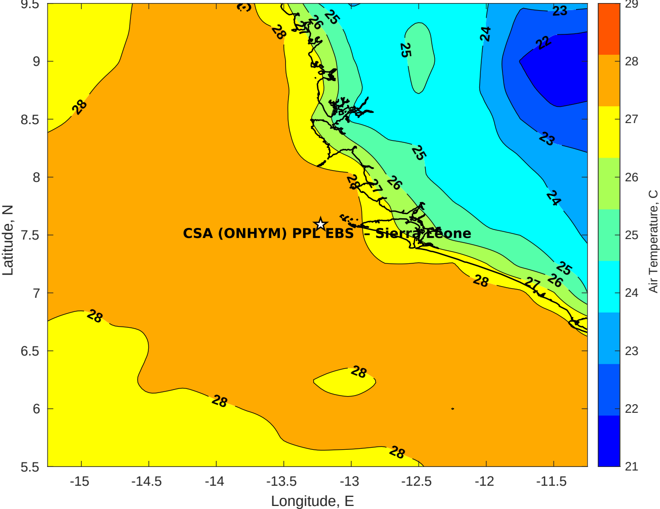
Air Temperature (C) for CSA (ONHYM) PPL EBS - Sierra Leone at 12-Dec-2025
