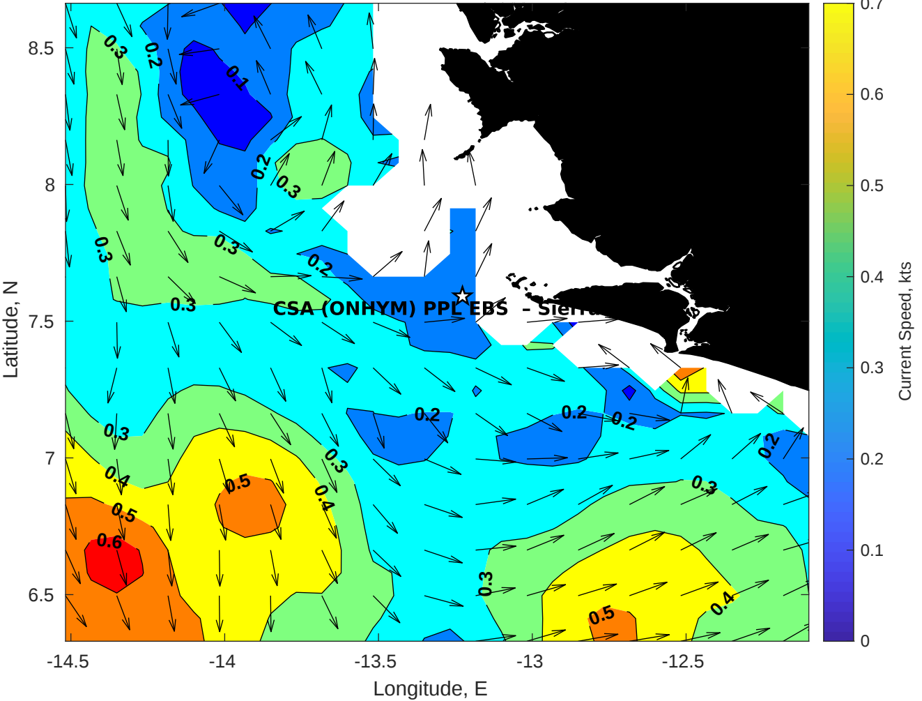
Surface Currents for CSA (ONHYM) PPL EBS - Sierra Leone at 11-Dec-2025 00:00:00
