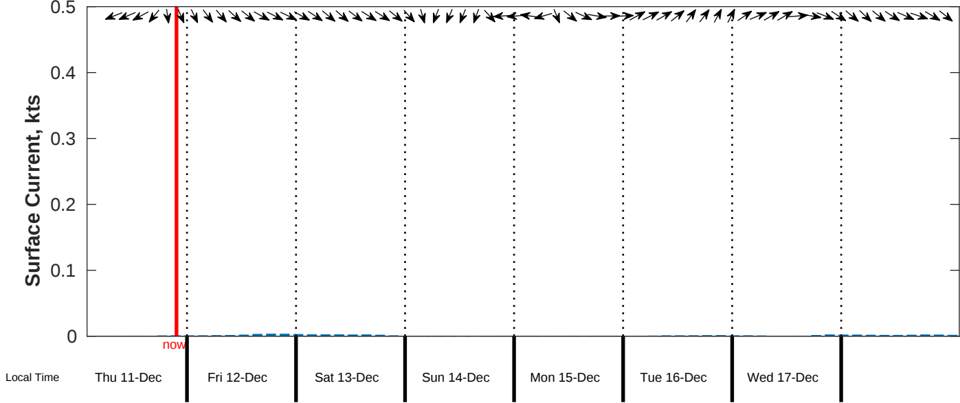
Surface Current Forecast for CSA (ONHYM) PPL EBS - Sierra Leone from 11-Dec-2025 00:00:00 to 19-Dec-2025 00:00:00
