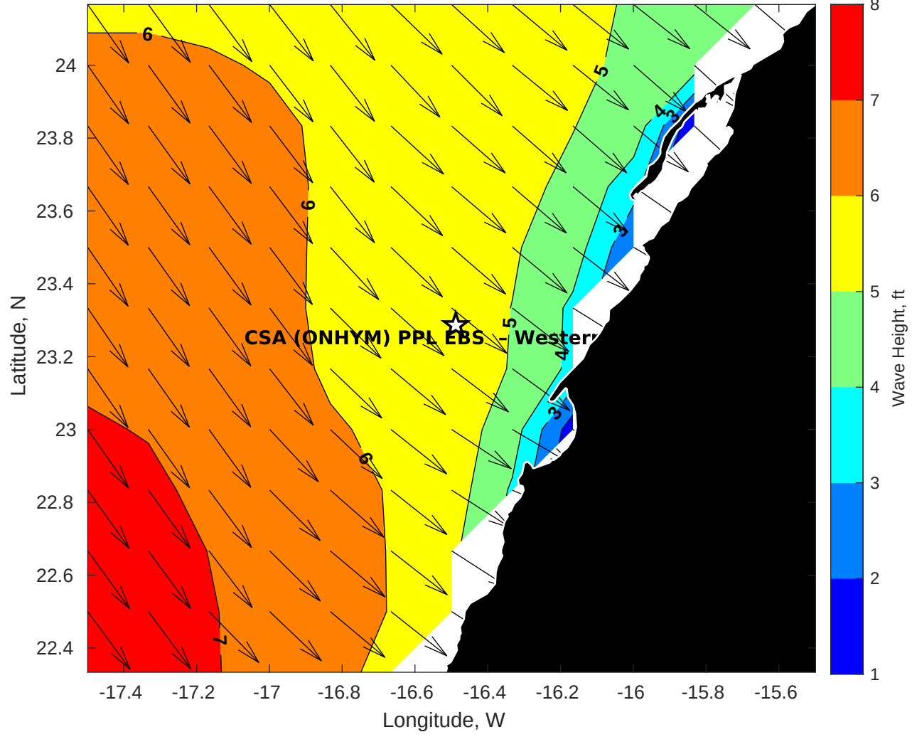
GFS Wave Height (ft) for CSA (ONHYM) PPL EBS - Western Sahara at 12-Dec-2025 09:00:00
