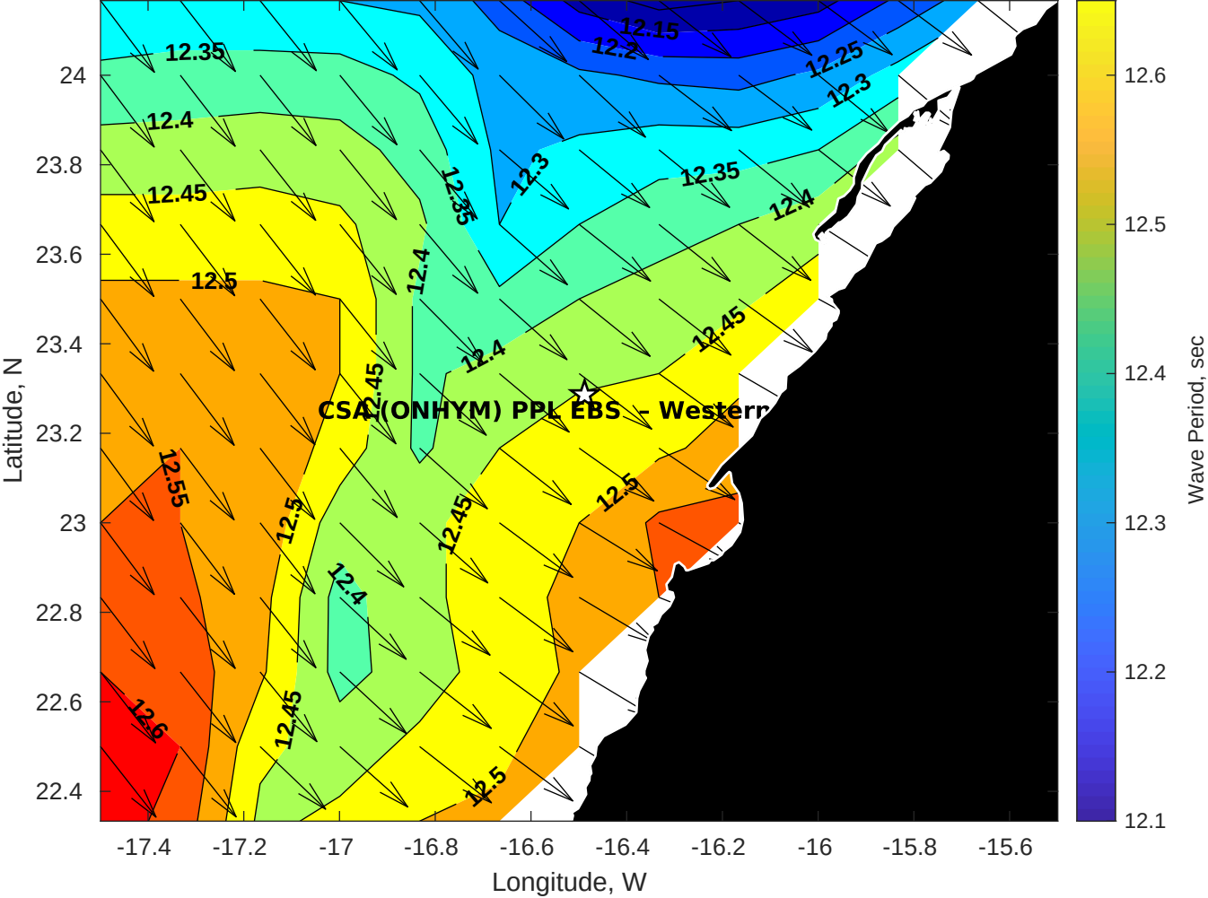
GFS Wave Period (sec) for CSA (ONHYM) PPL EBS - Western Sahara at 12-Dec-2025 09:00:00
