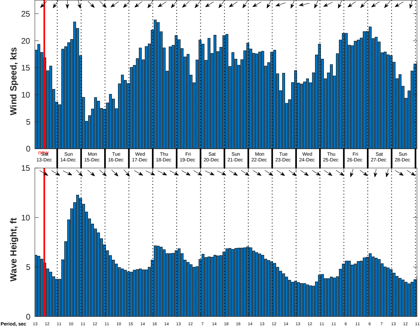
Wind & Wave Forecast for CSA (ONHYM) PPL EBS - Western Sahara from 12-Dec-2025 01:00:00 to 28-Dec-2025 01:00:00
