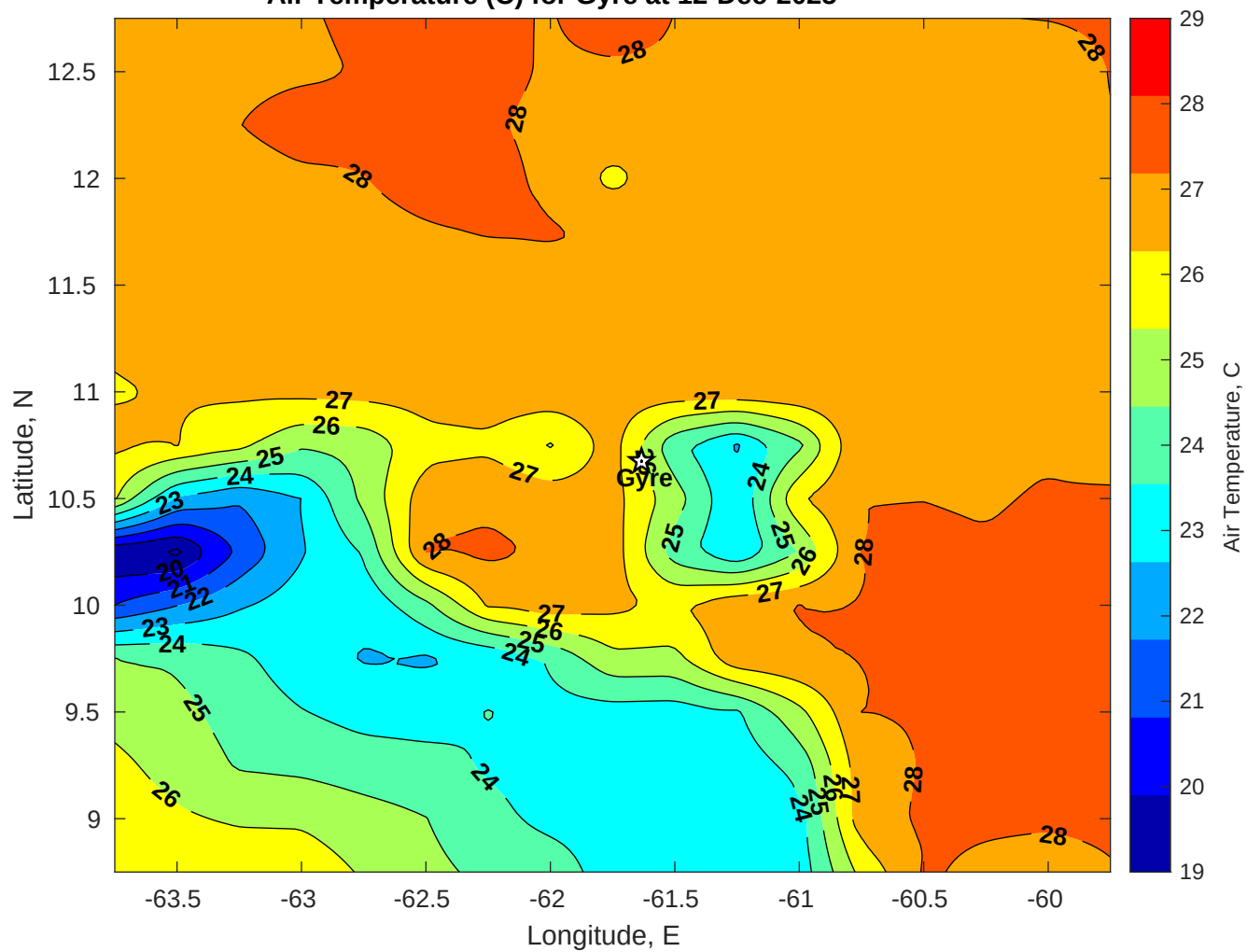
Air Temperature (C) for Gyre at 12-Dec-2025
