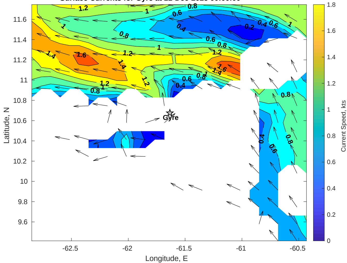
Surface Currents for Gyre at 11-Dec-2025 00:00:00
