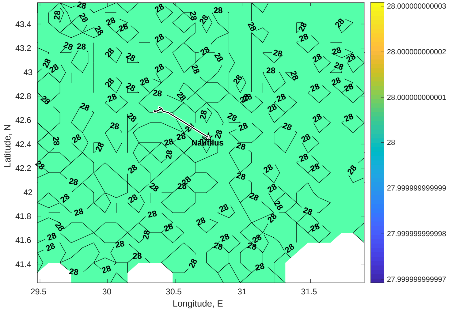
Surface Salinity for Nautilus at 11-Dec-2025 00:00:00
