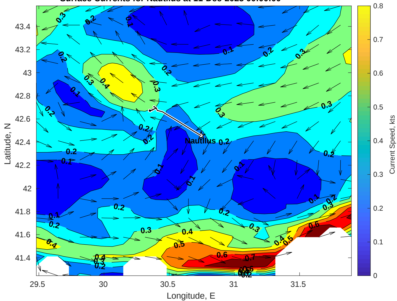
Surface Currents for Nautilus at 11-Dec-2025 00:00:00
