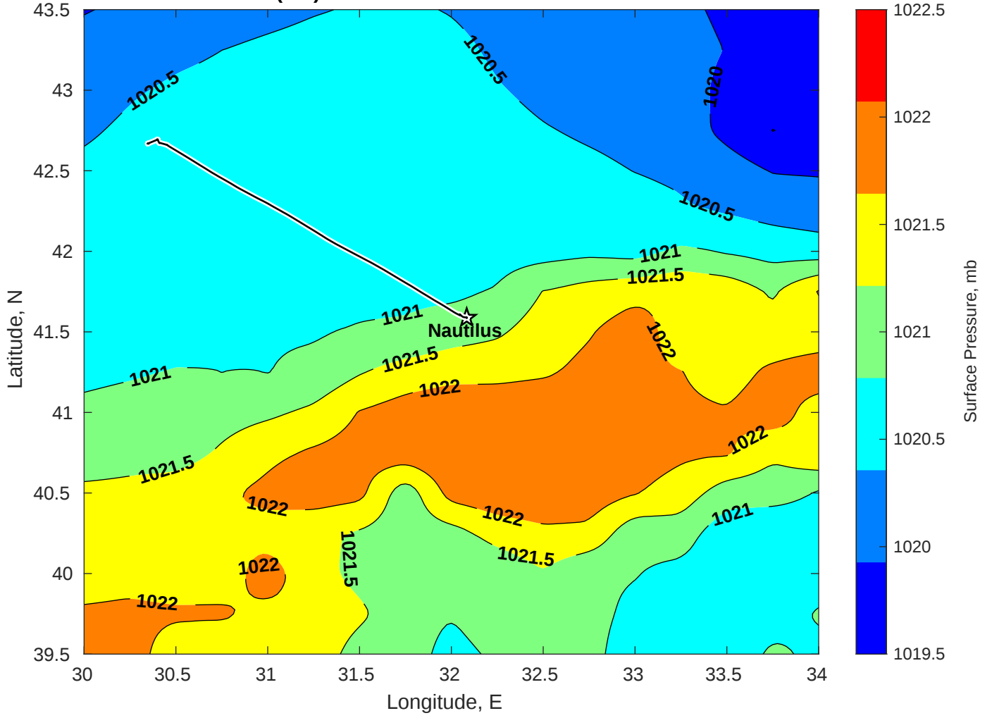
Surface Pressure (mb) for Nautilus at 12-Dec-2025 00:00:00
