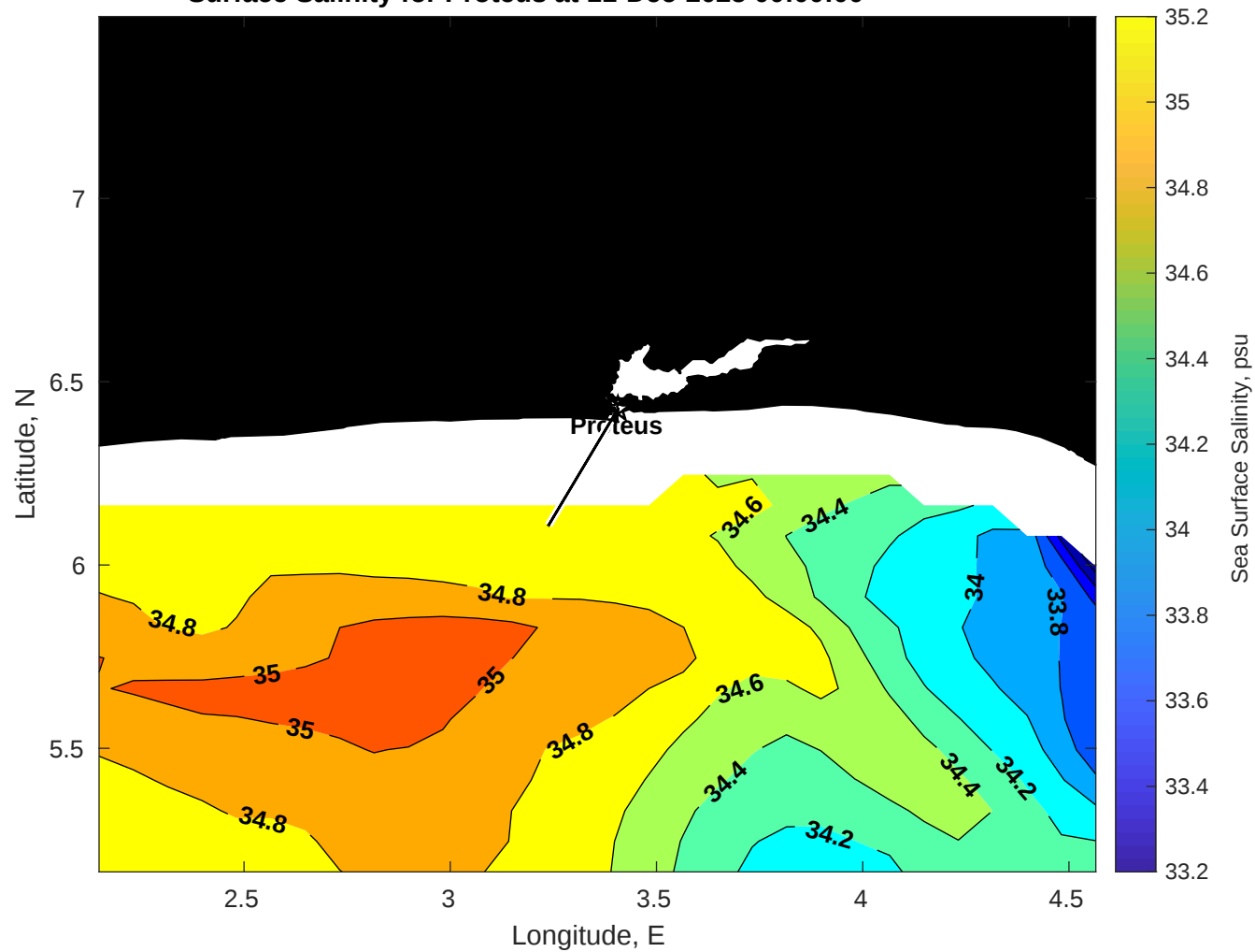
Surface Salinity for Proteus at 11-Dec-2025 00:00:00
