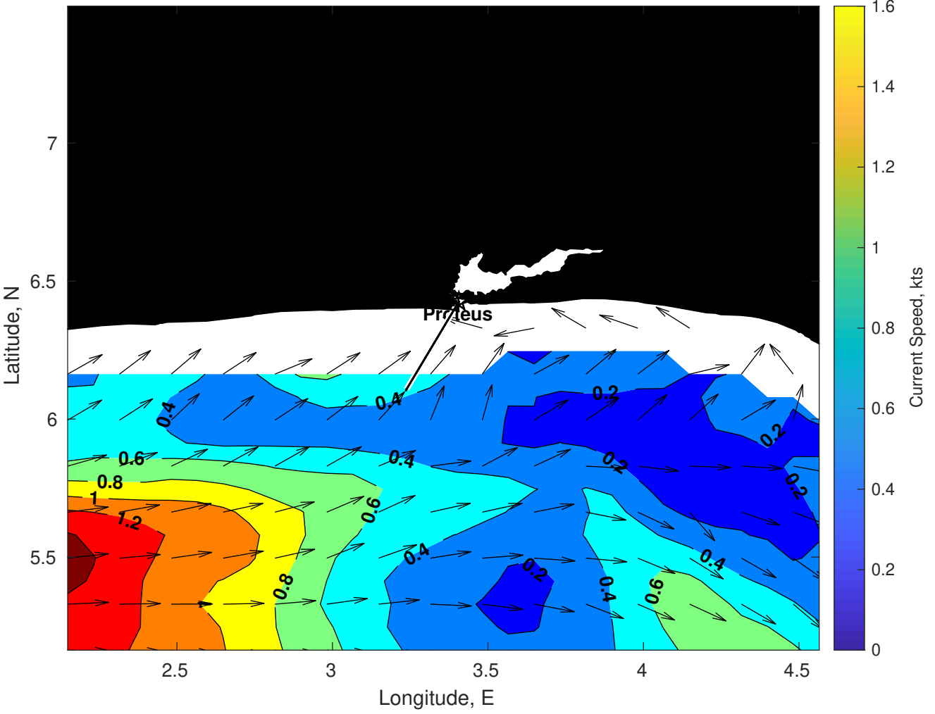
Surface Currents for Proteus at 11-Dec-2025 00:00:00
