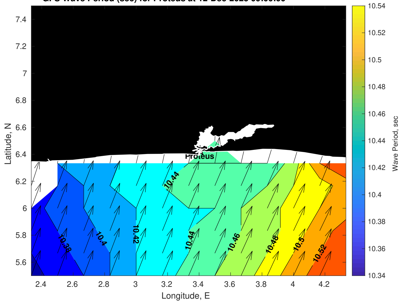
GFS Wave Period (sec) for Proteus at 12-Dec-2025 09:00:00
