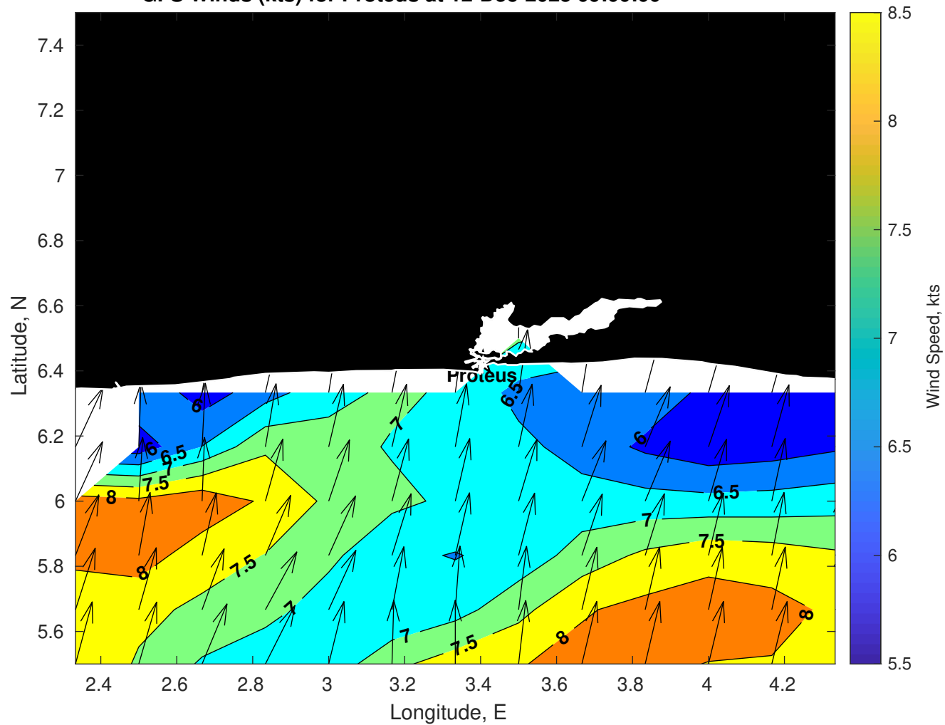
GFS Winds (kts) for Proteus at 12-Dec-2025 09:00:00
