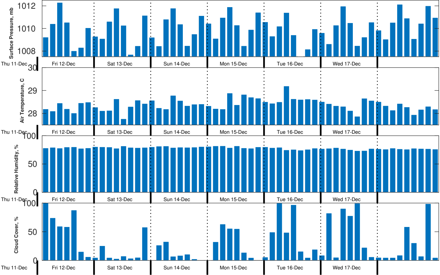
Met Forecast for Proteus from 12-Dec-2025 00:00:00 to 19-Dec-2025 00:00:00
