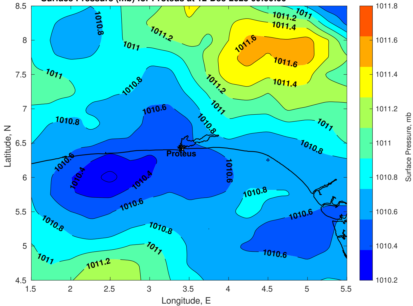
Surface Pressure (mb) for Proteus at 12-Dec-2025 00:00:00
