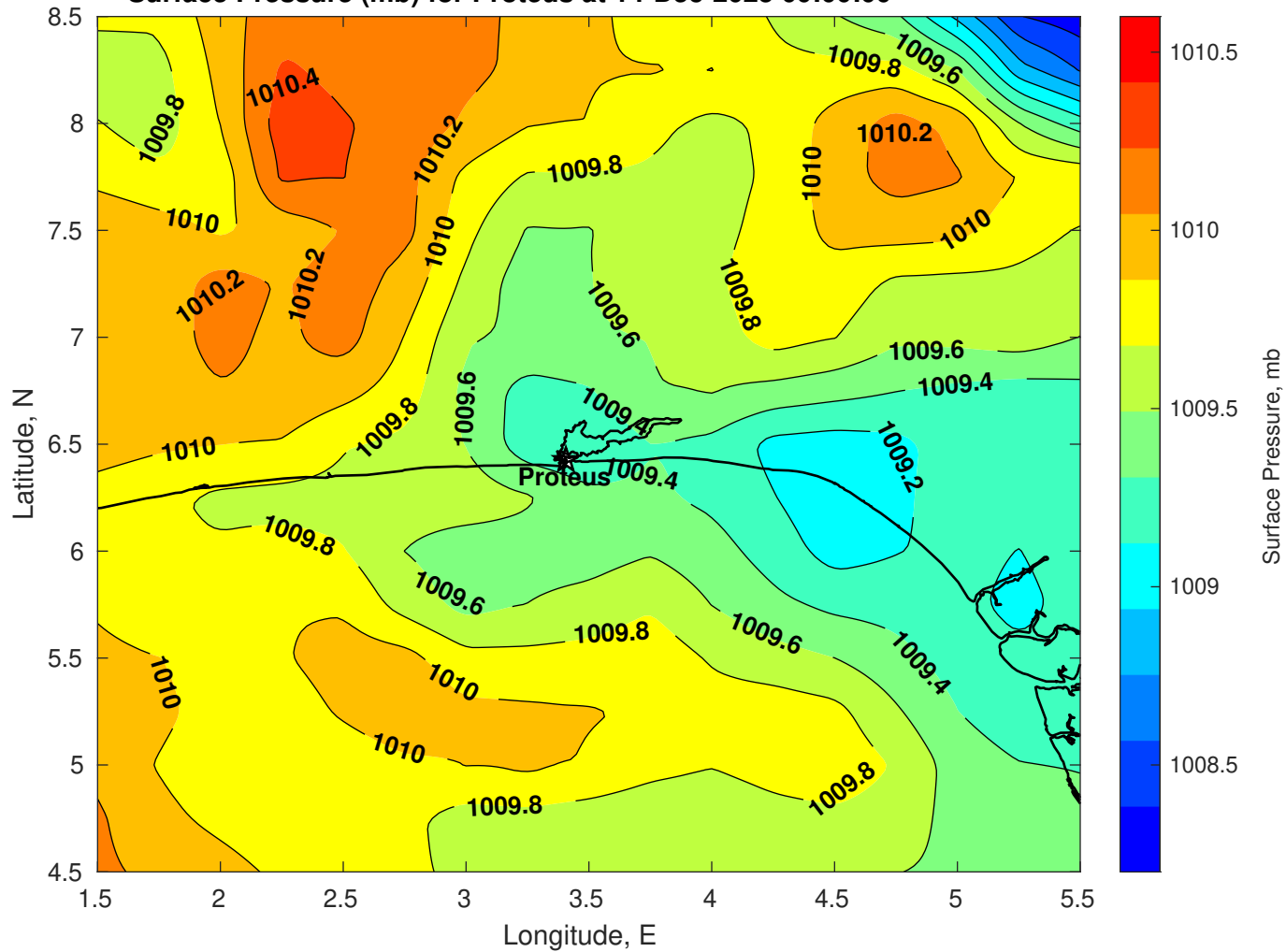
Surface Pressure (mb) for Proteus at 14-Dec-2025 00:00:00
