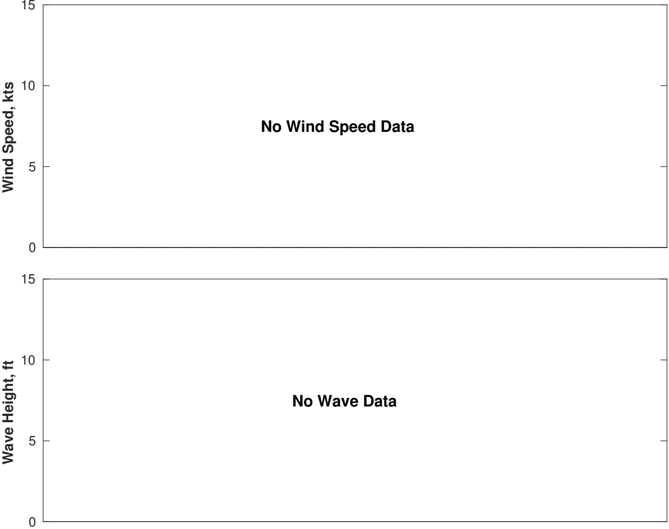
Wind & Wave Forecast for Proteus from 12-Dec-2025 01:00:00 to 28-Dec-2025 01:00:00
