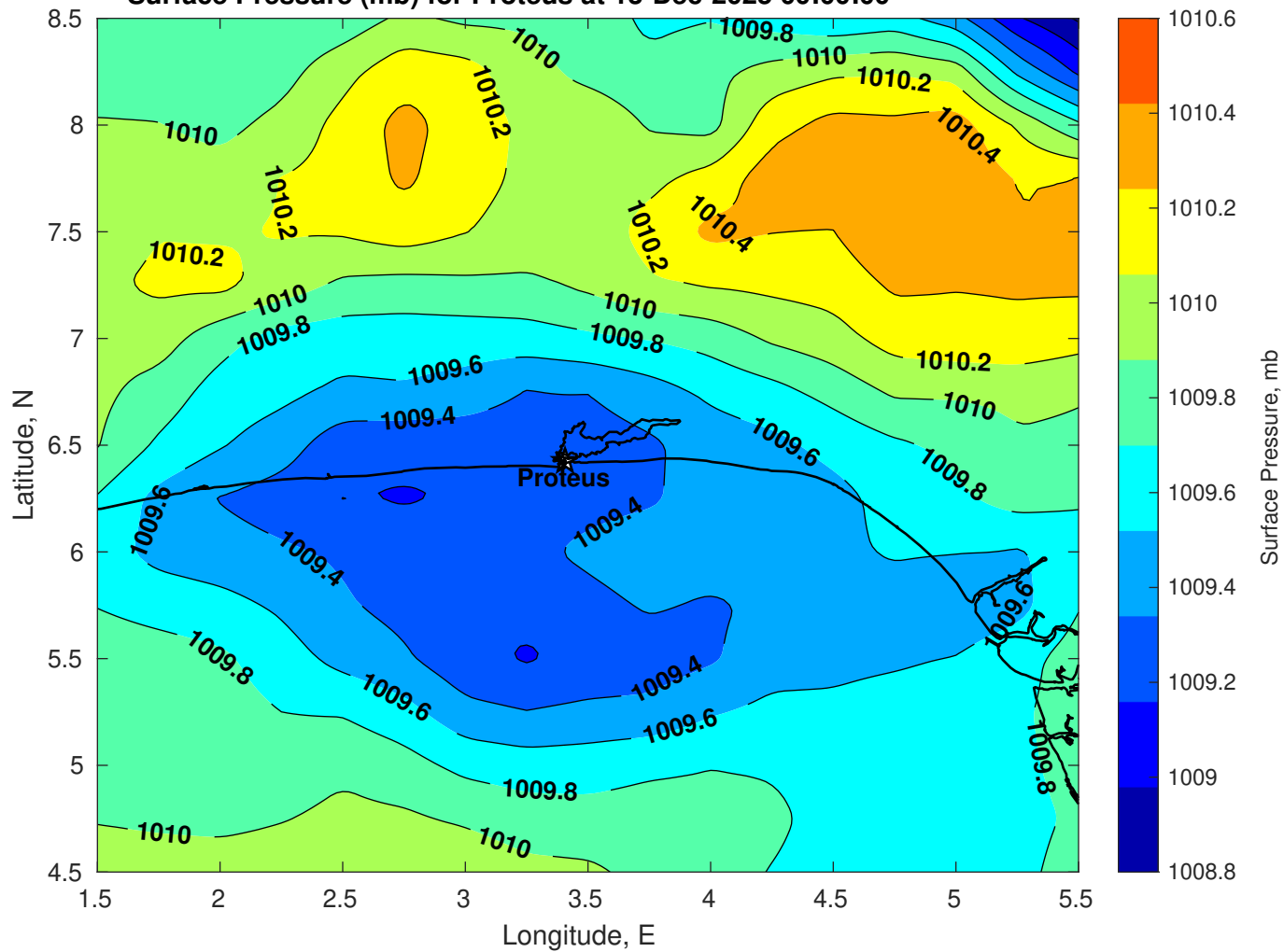
Surface Pressure (mb) for Proteus at 13-Dec-2025 00:00:00
