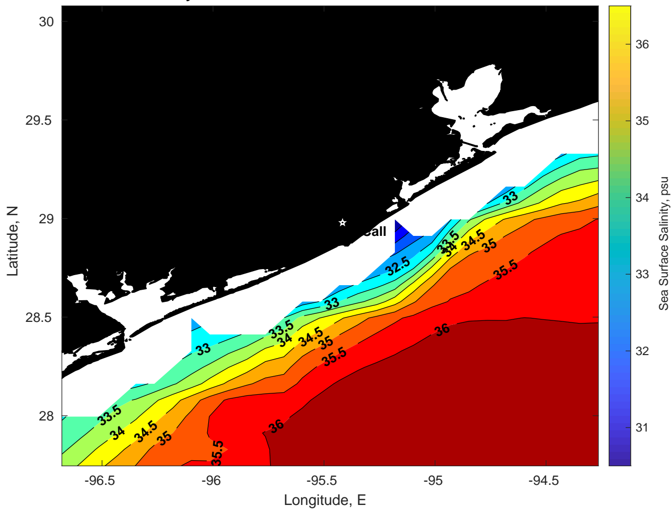
Surface Salinity for Brooks McCall at 12-Dec-2025 00:00:00
