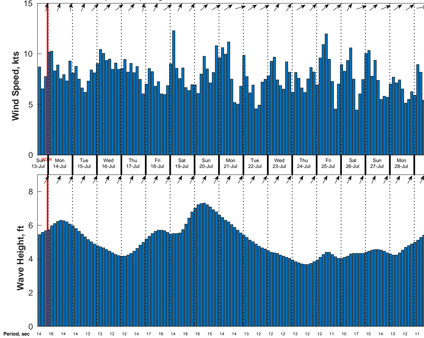
Wind & Wave Forecast for CABGOC (Chevron) Angola BLK 14 EBS from 13-Jul-2025 14:00:00 to 29-Jul-2025 14:00:00
