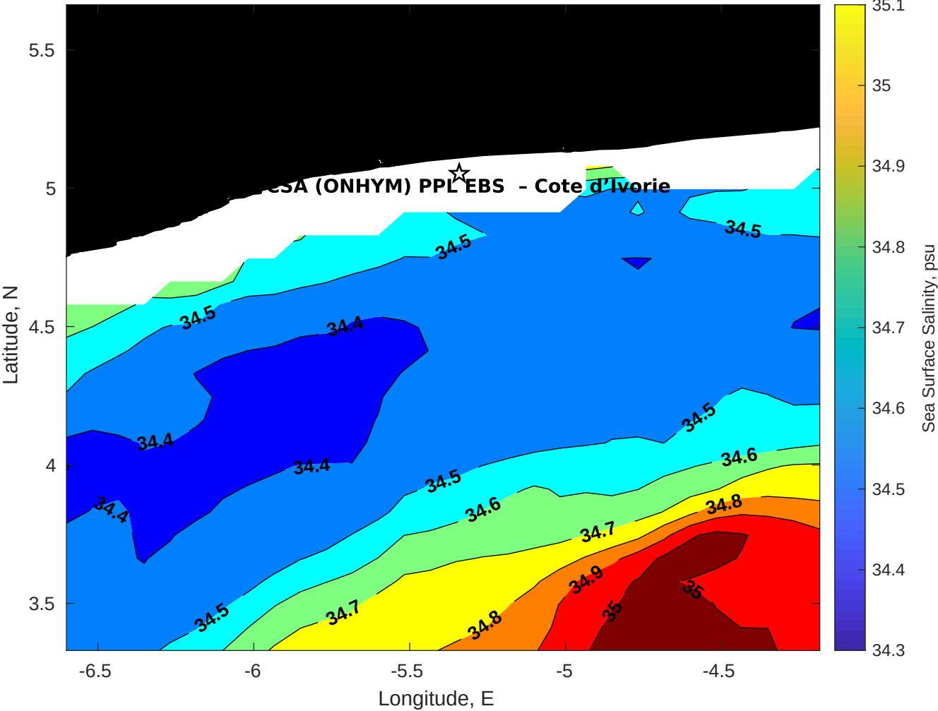
Surface Salinity for CSA (ONHYM) PPL EBS - Cote d'Ivoire at 12-Dec-2025 00:00:00
