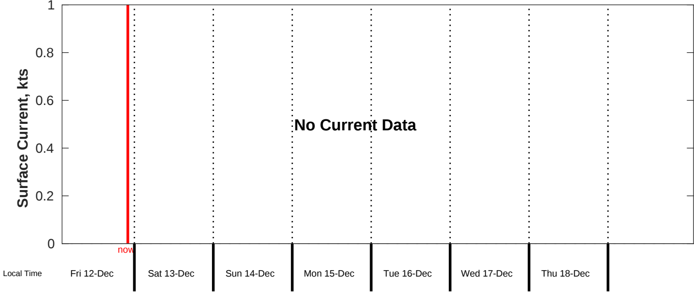
Surface Current Forecast for CSA (ONHYM) PPL EBS - Cote d'Ivoire from 12-Dec-2025 00:00:00 to 20-Dec-2025 00:00:00
