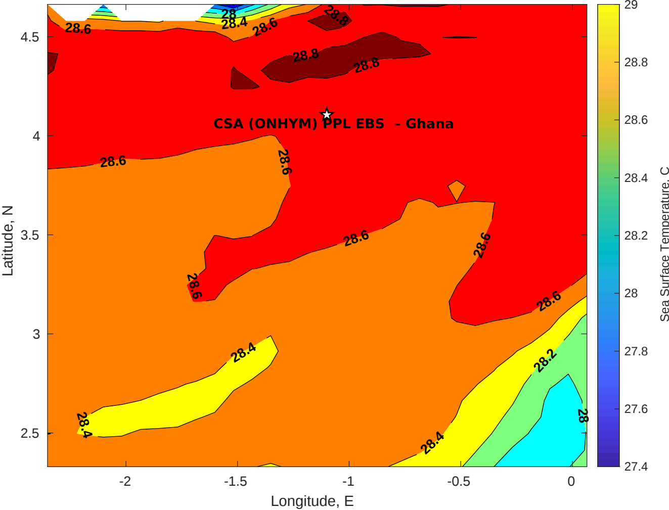
SST for CSA (ONHYM) PPL EBS - Ghana at 12-Dec-2025 00:00:00
