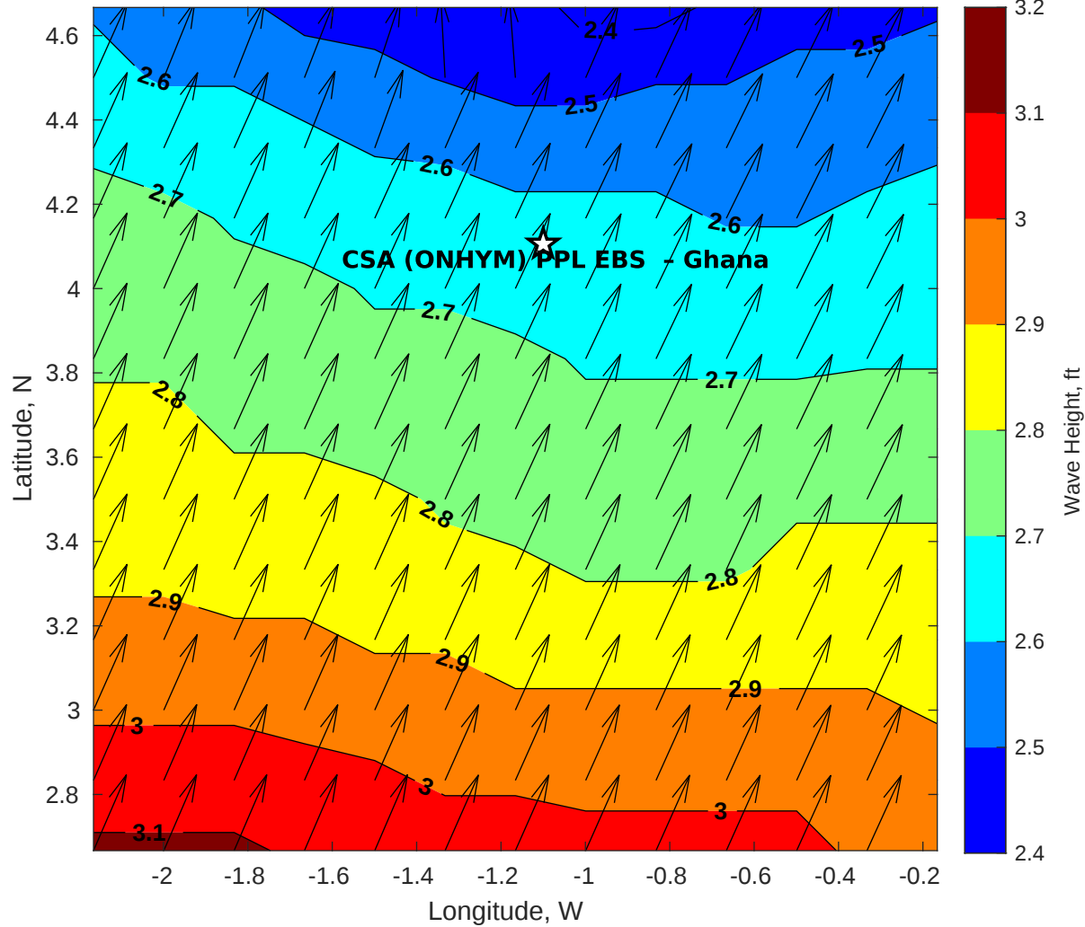
GFS Wave Height (ft) for CSA (ONHYM) PPL EBS - Ghana at 13-Dec-2025 09:00:00
