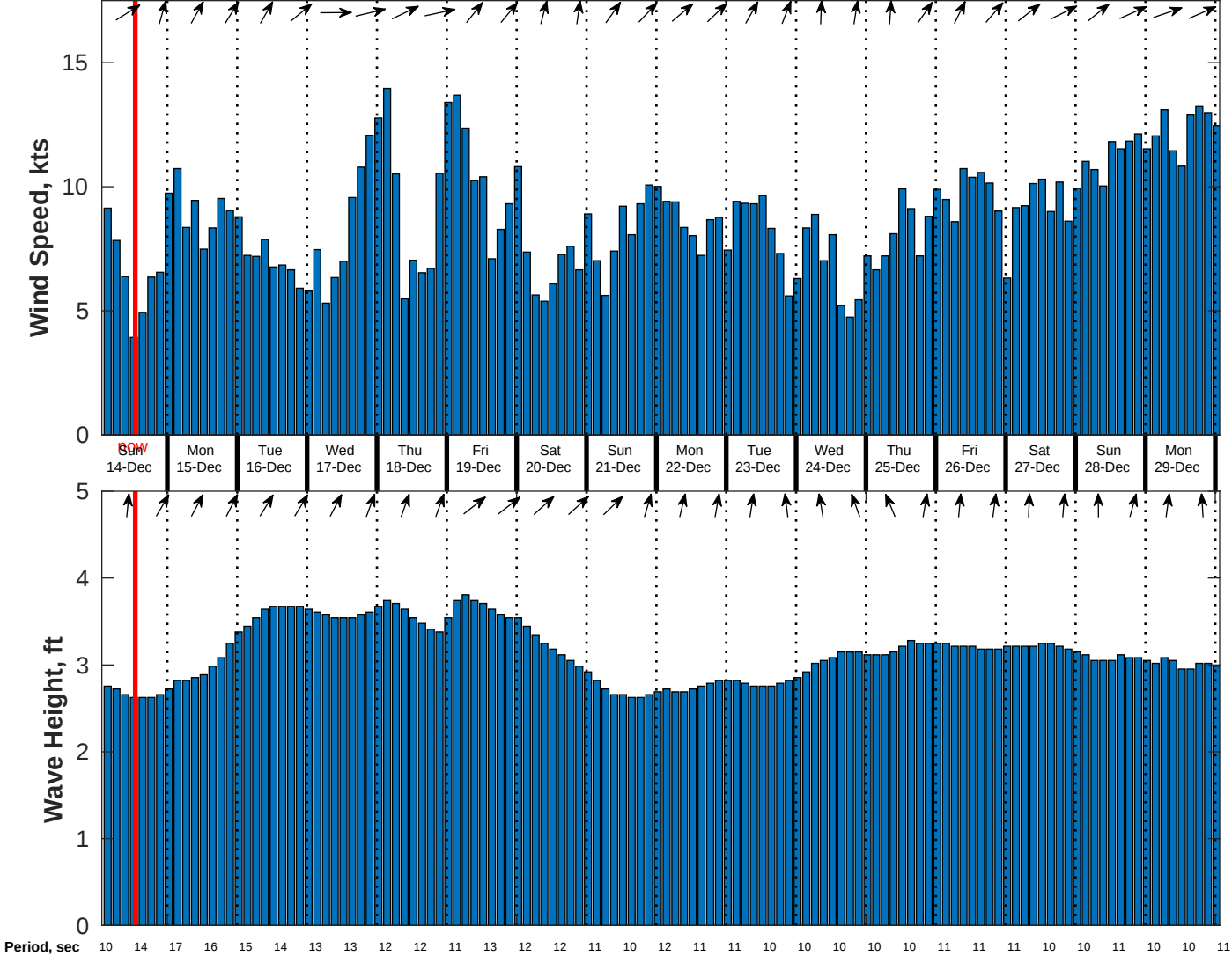
Wind & Wave Forecast for CSA (ONHYM) PPL EBS - Ghana from 13-Dec-2025 02:00:00 to 29-Dec-2025 02:00:00
