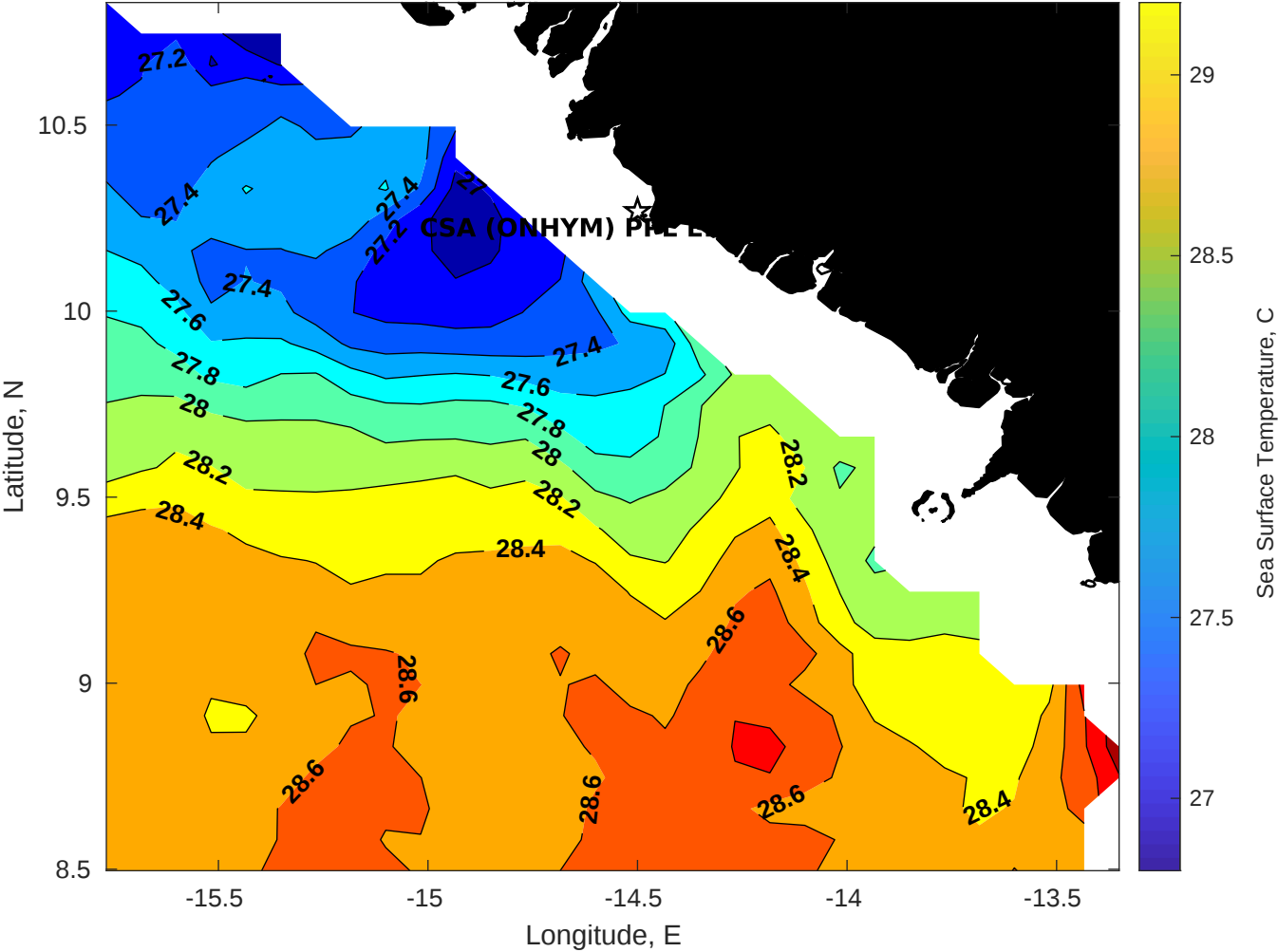
SST for CSA (ONHYM) PPL EBS - Guinea at 12-Dec-2025 00:00:00
