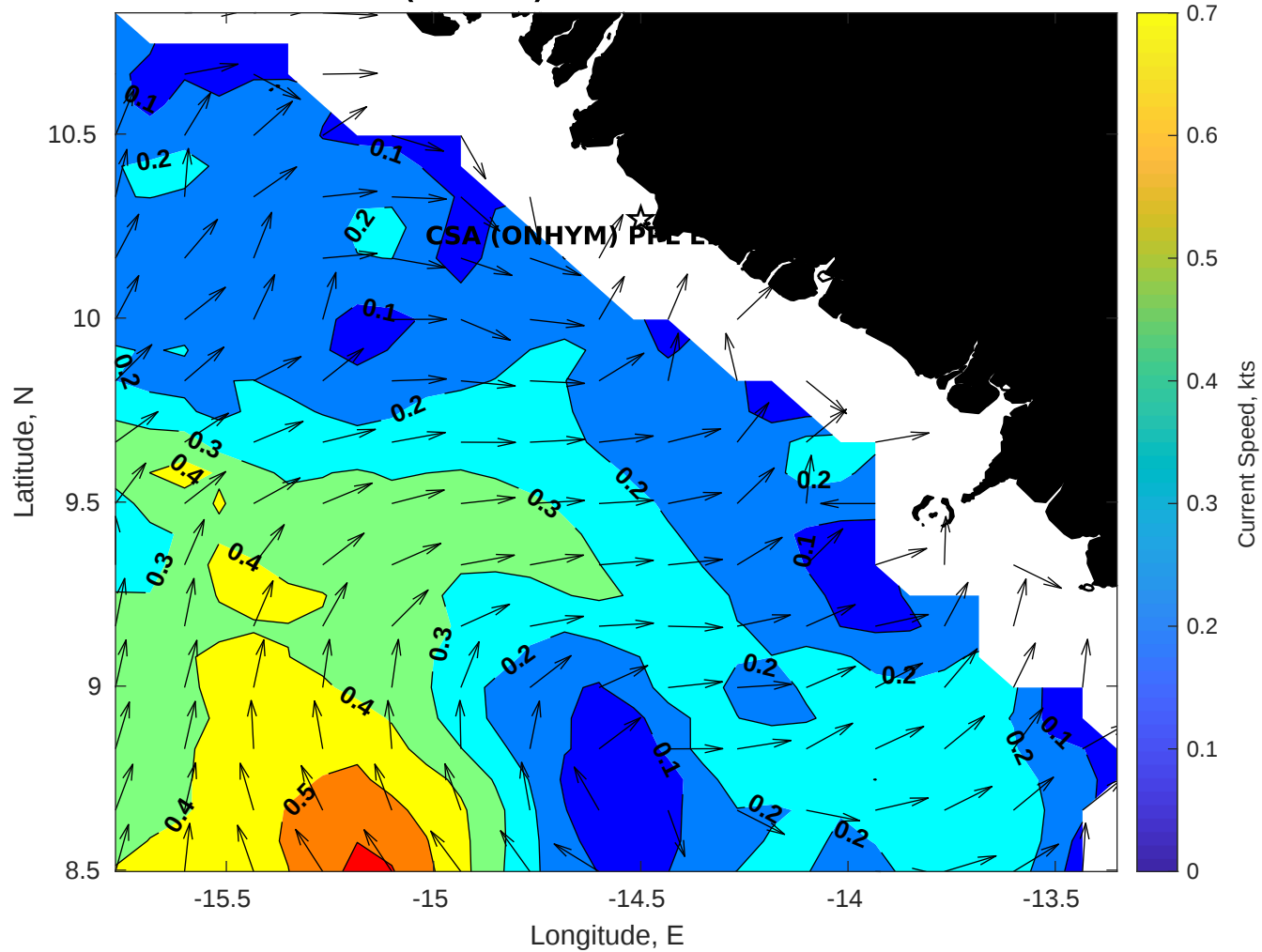
Surface Currents for CSA (ONHYM) PPL EBS - Guinea at 12-Dec-2025 00:00:00
