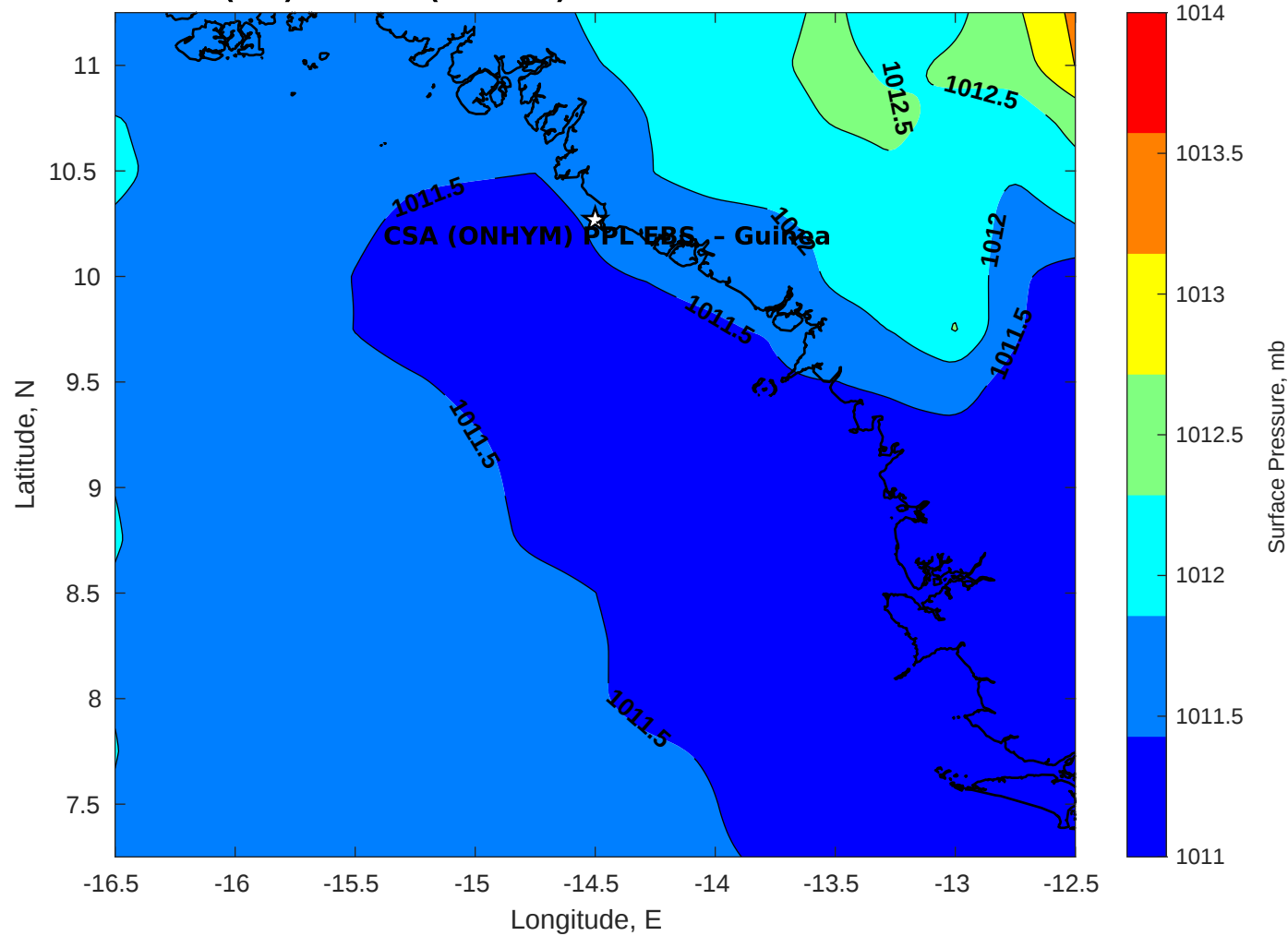
Surface Pressure (mb) for CSA (ONHYM) PPL EBS - Guinea at 13-Dec-2025 00:00:00
