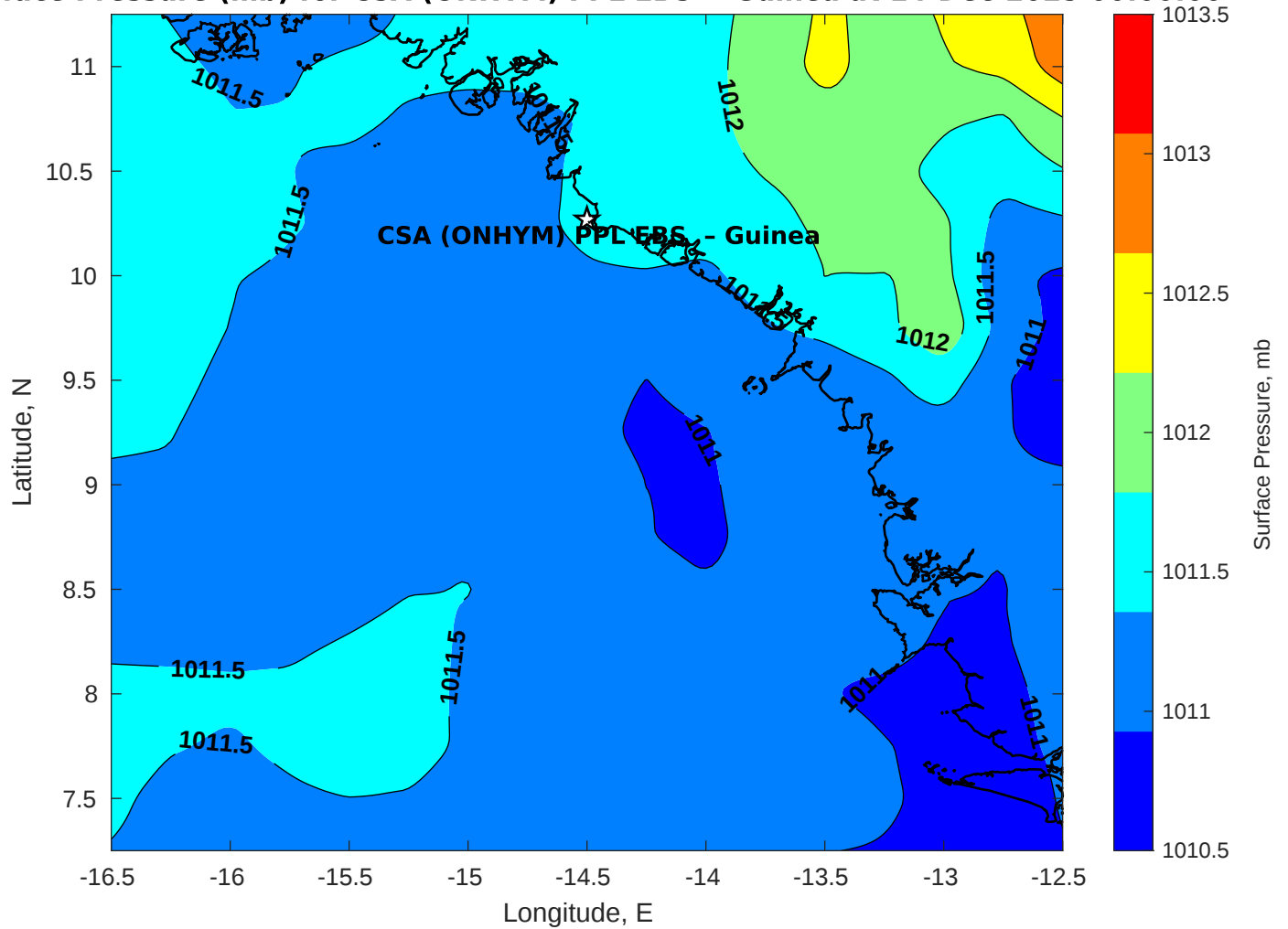
Surface Pressure (mb) for CSA (ONHYM) PPL EBS - Guinea at 14-Dec-2025 00:00:00
