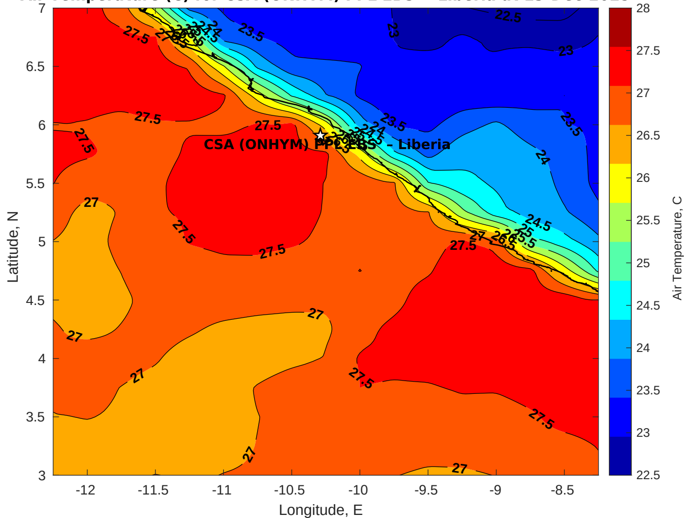
Air Temperature (C) for CSA (ONHYM) PPL EBS - Liberia at 13-Dec-2025
