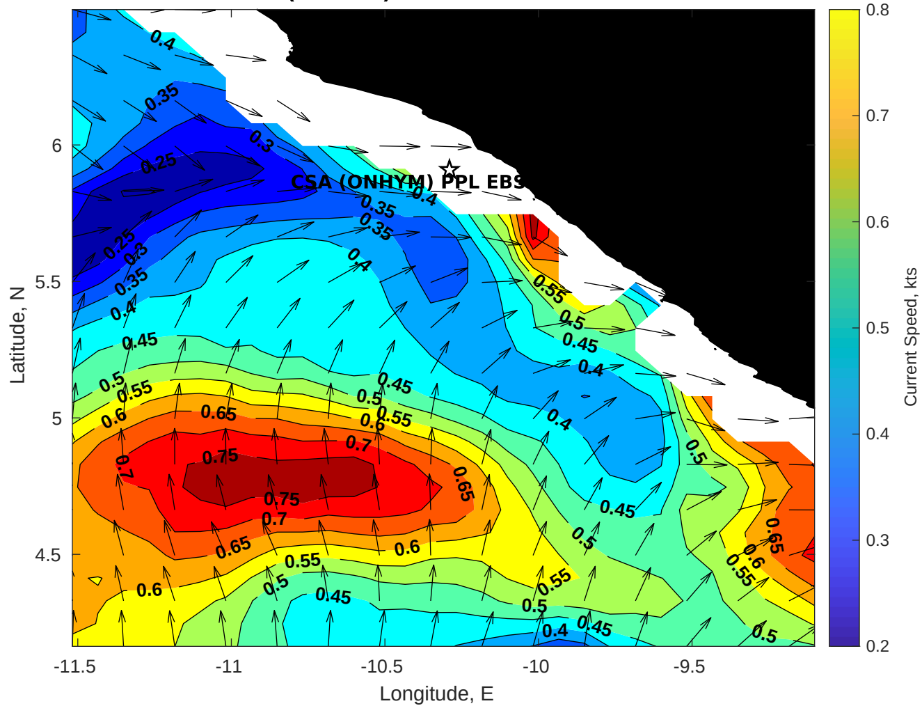
Surface Currents for CSA (ONHYM) PPL EBS - Liberia at 12-Dec-2025 00:00:00
