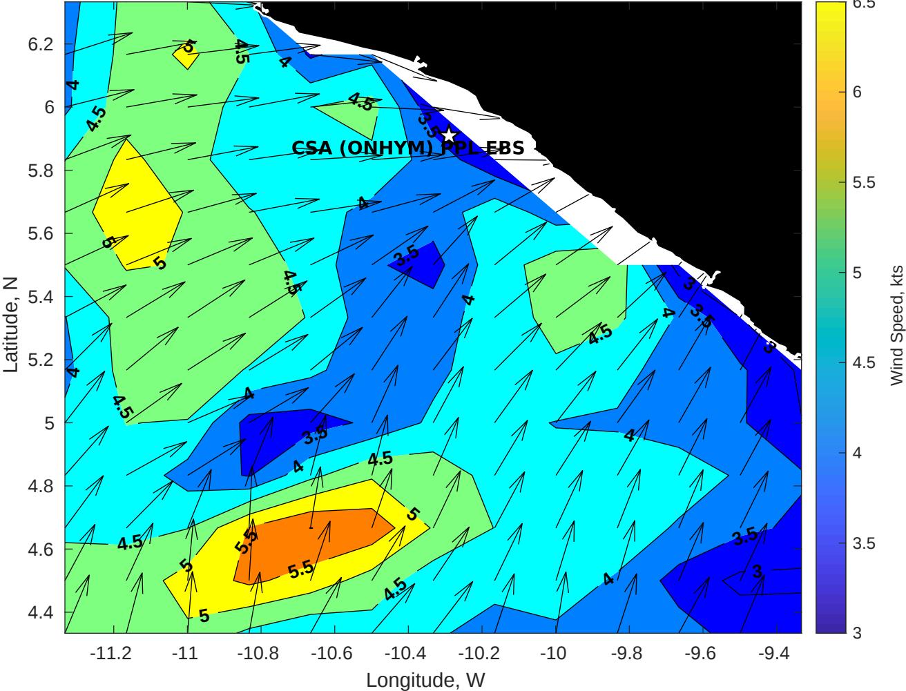
GFS Winds (kts) for CSA (ONHYM) PPL EBS - Liberia at 13-Dec-2025 09:00:00
