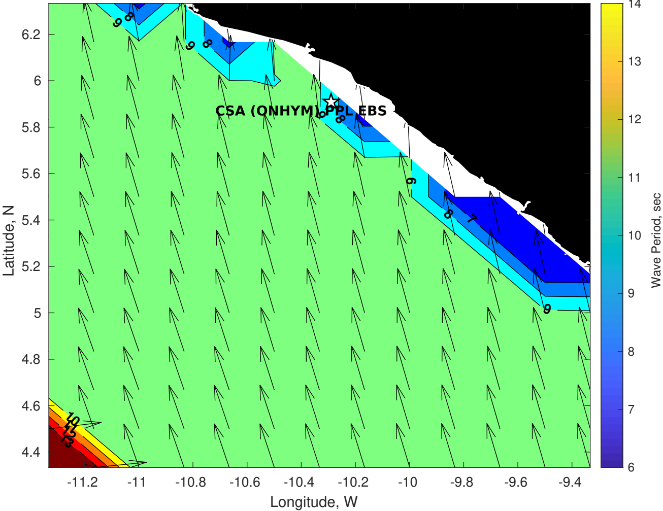
GFS Wave Period (sec) for CSA (ONHYM) PPL EBS - Liberia at 13-Dec-2025 09:00:00
