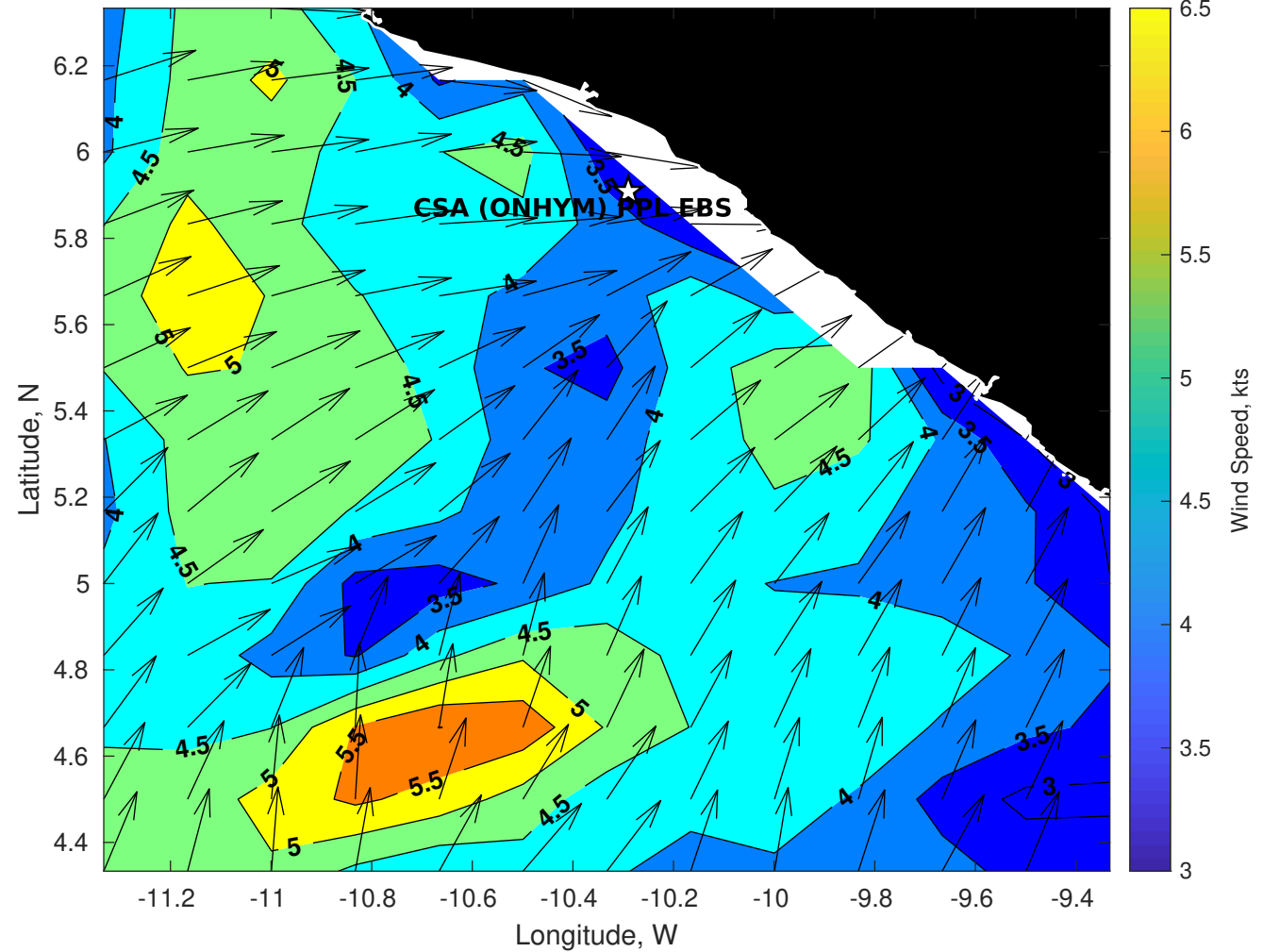
GFS Winds (kts) for CSA (ONHYM) PPL EBS - Liberia at 13-Dec-2025 09:00:00
