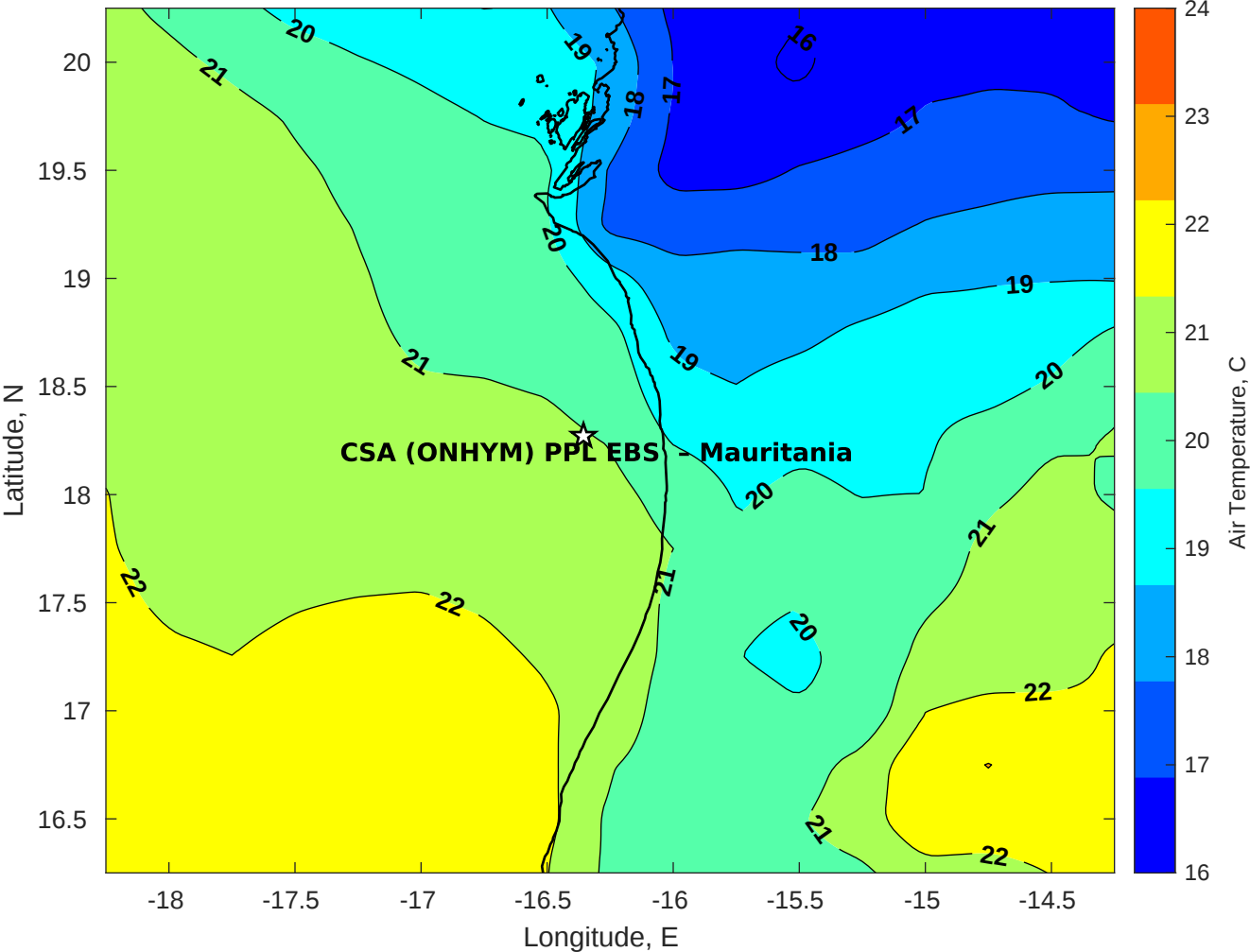
Air Temperature (C) for CSA (ONHYM) PPL EBS - Mauritania at 13-Dec-2025
