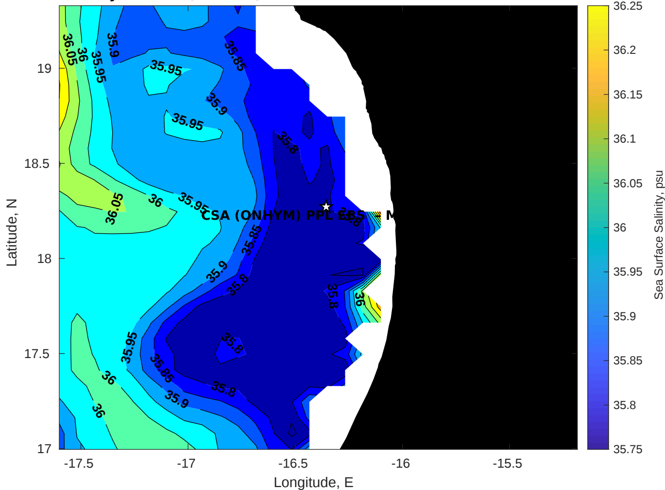
Surface Salinity for CSA (ONHYM) PPL EBS - Mauritania at 12-Dec-2025 00:00:00
